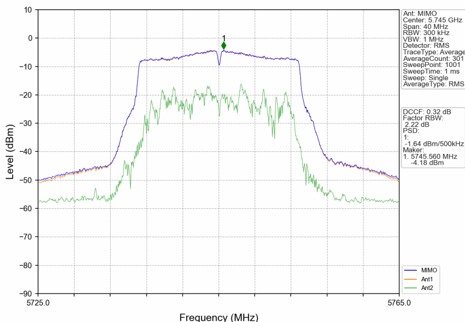
802.11ac(VHT20)_LCH_5745MHz_MIMO_NTNV
