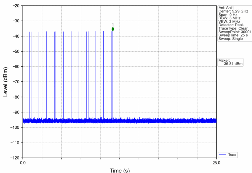
Signal Calibration_802.11ac(VHT80)_2A_5290MHz_RadarType0_Trial0
