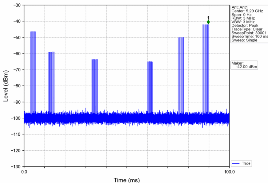
Signal Calibration_802.11ac(VHT80)_2A_5290MHz_RadarType0_Trial0
