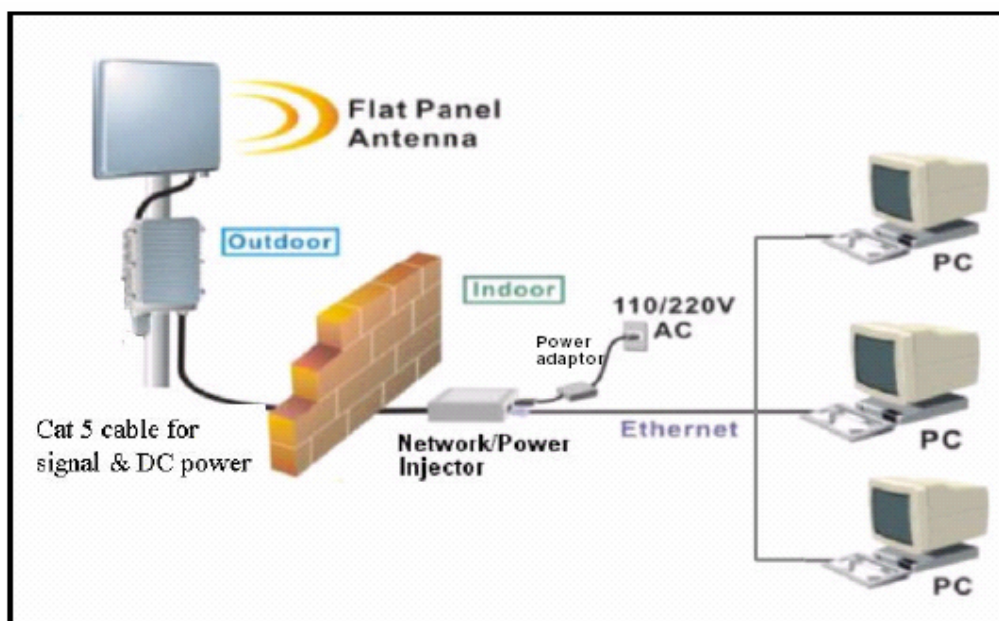
Figure 2-14 Physical Installation of GateOne 240G with flat panel antenna
