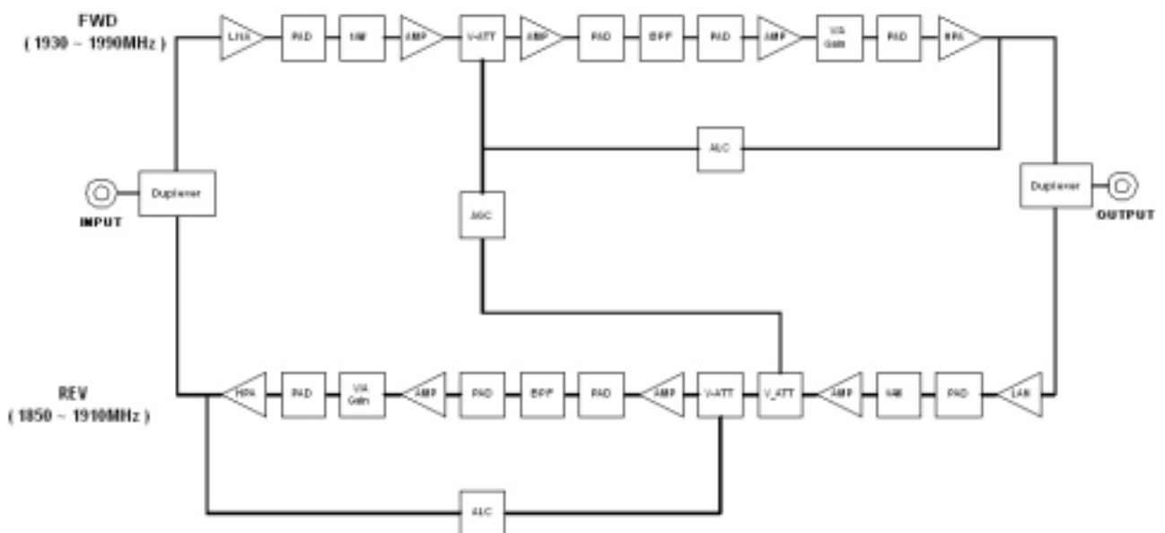
Block Diagram
