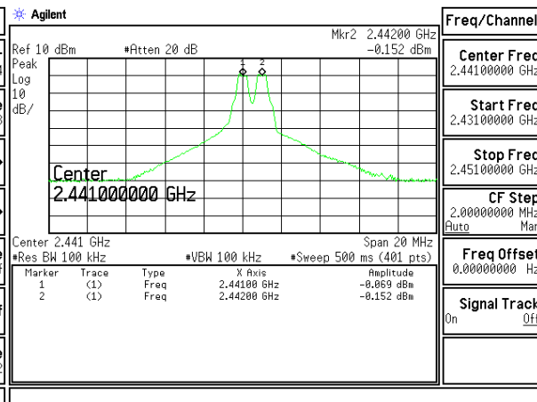
Channel 39 2441MHz
