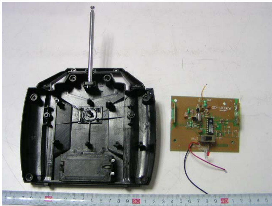
EUT- Inside View (3)
