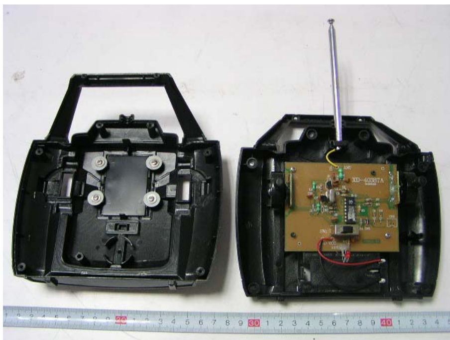
EUT-Inside View (1)
