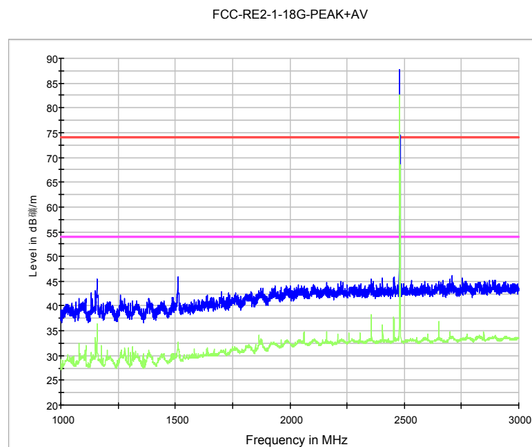
Fig. 48 Radiated Spurious Emission (GFSK, Ch78, 1 GHz ~3 GHz)
