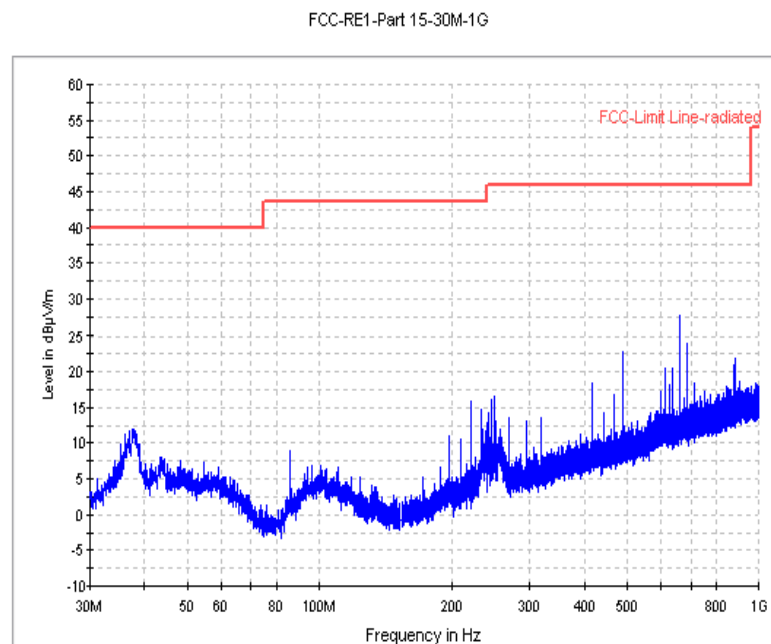
Fig. 47 Radiated Spurious Emission (GFSK, Ch78, 30 MHz ~1 GHz)
