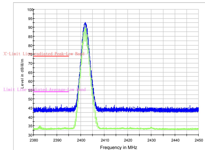
FCC-RE2-BAND Edge-Low Band
