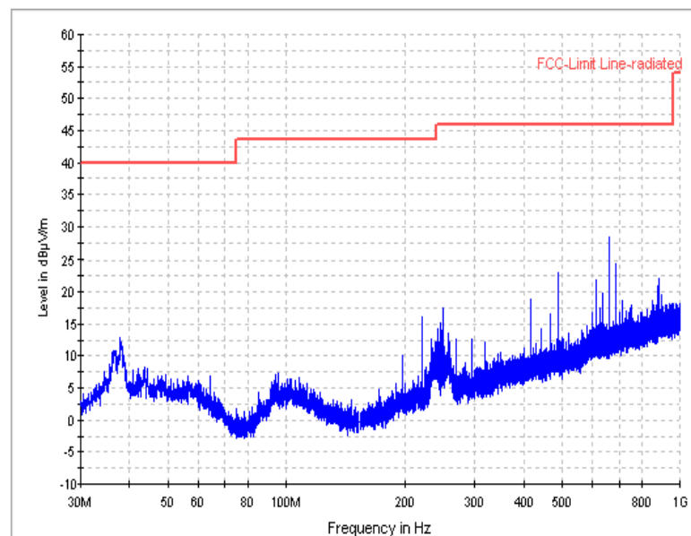
FCC-RE1-Part 15-30M-1G
