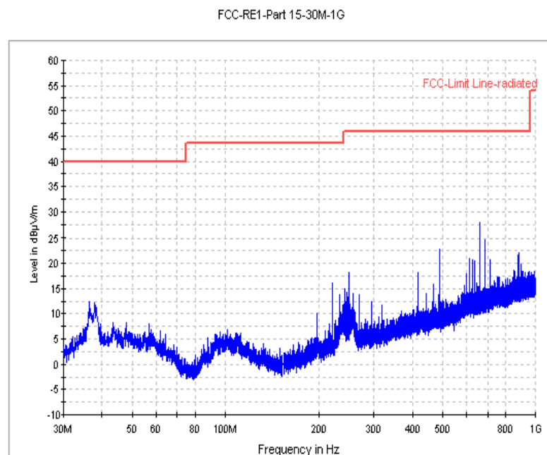
Fig. 70 Radiated Spurious Emission (802.11g, Ch11, 30MHz-1 GHz)
