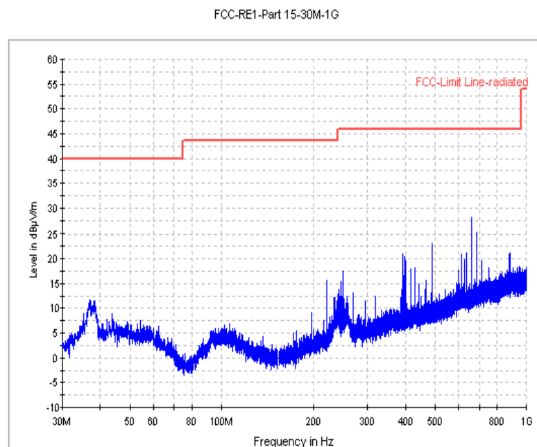
Fig. 78 Radiated Spurious Emission (802.11n-20M, Ch6, 30MHz-1 GHz)
