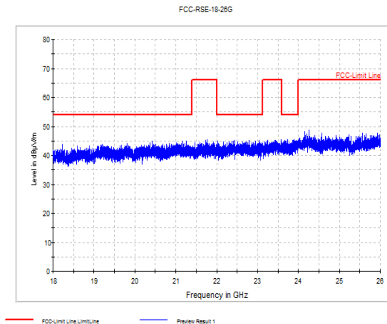
Fig. 86 Radiated emission: 18 GHz - 26 GHz
