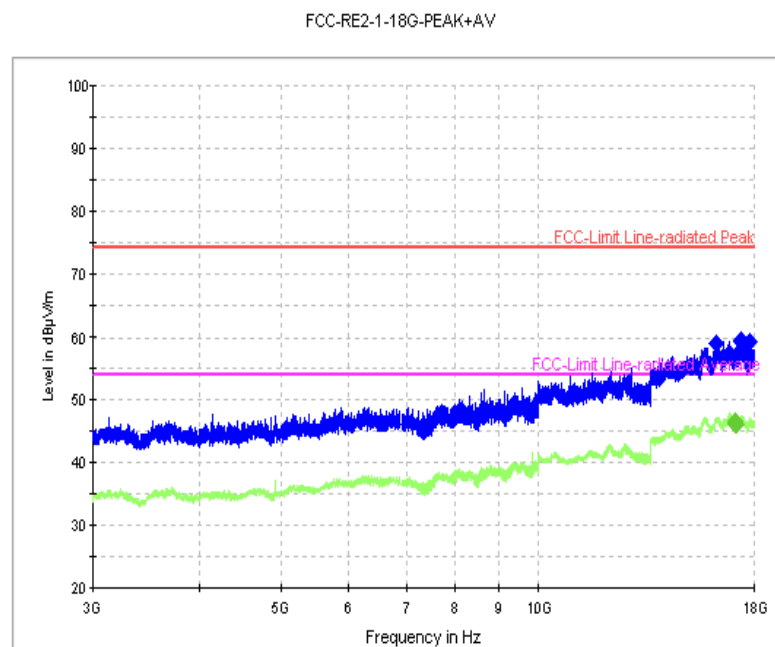
Fig. 72 Radiated Spurious Emission (802.11g, Ch11, 3 GHz-18 GHz)
