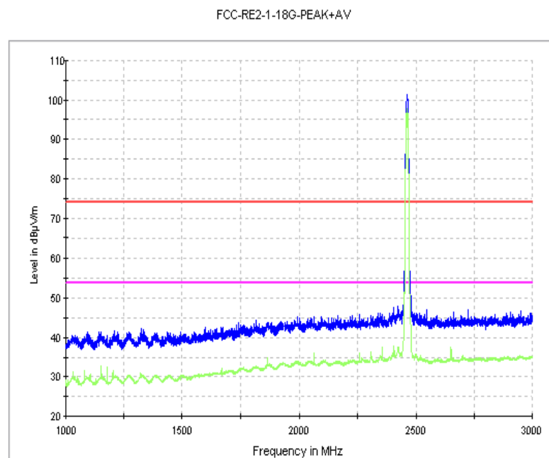
Fig. 60 Radiated Spurious Emission (802.11b, Ch11, 1 GHz-3 GHz)
