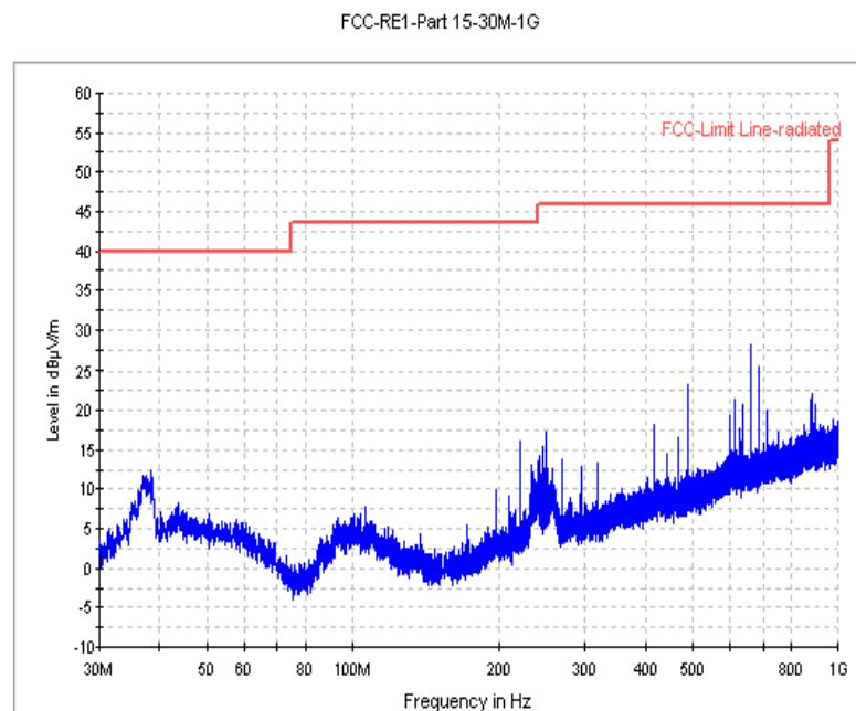
Fig. 67 Radiated Spurious Emission (802.11g, Ch6, 30MHz-1 GHz)
