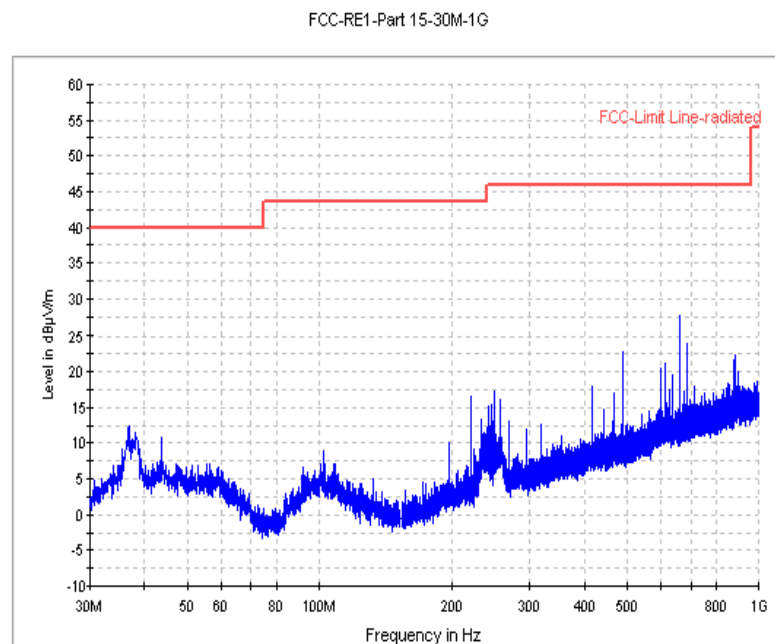
Fig. 81 Radiated Spurious Emission (802.11n-20M, Ch11, 30MHz-1 GHz)
