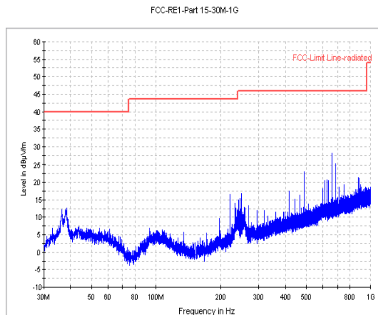
Fig. 64 Radiated Spurious Emission (802.11g, Ch1,30MHz-1 GHz)
