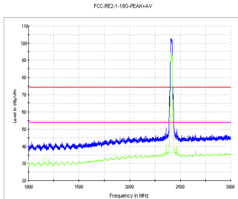
Fig. 65 Radiated Spurious Emission (802.11g, Ch1, 1 GHz-3 GHz)
