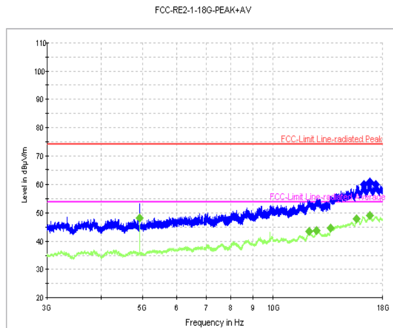
Fig. 61 Radiated Spurious Emission (802.11b, Ch11, 3 GHz-18 GHz)
