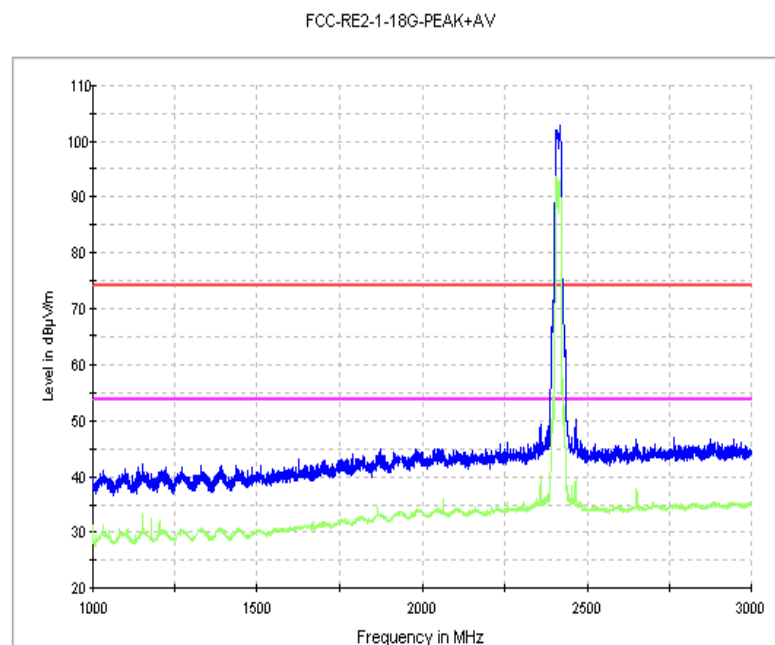
Fig. 68 Radiated Spurious Emission (802.11g, Ch6, 1 GHz-3 GHz)
