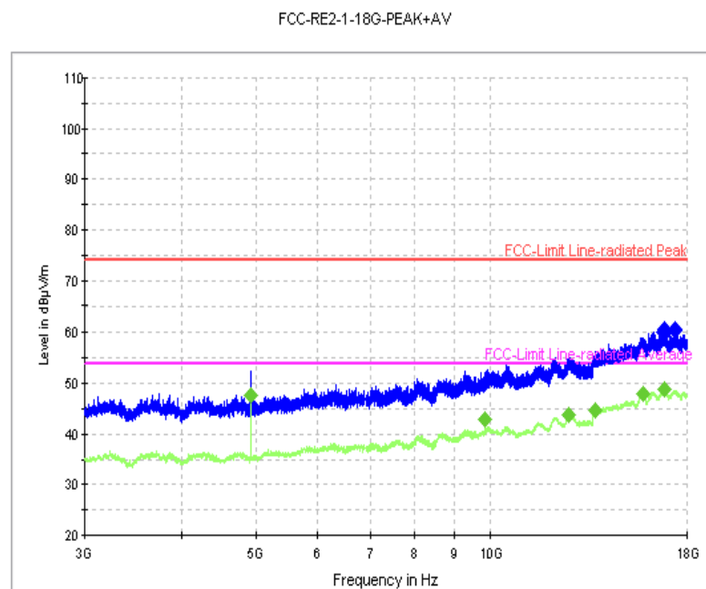
Fig. 58 Radiated Spurious Emission (802.11b, Ch6, 3 GHz-18 GHz)
