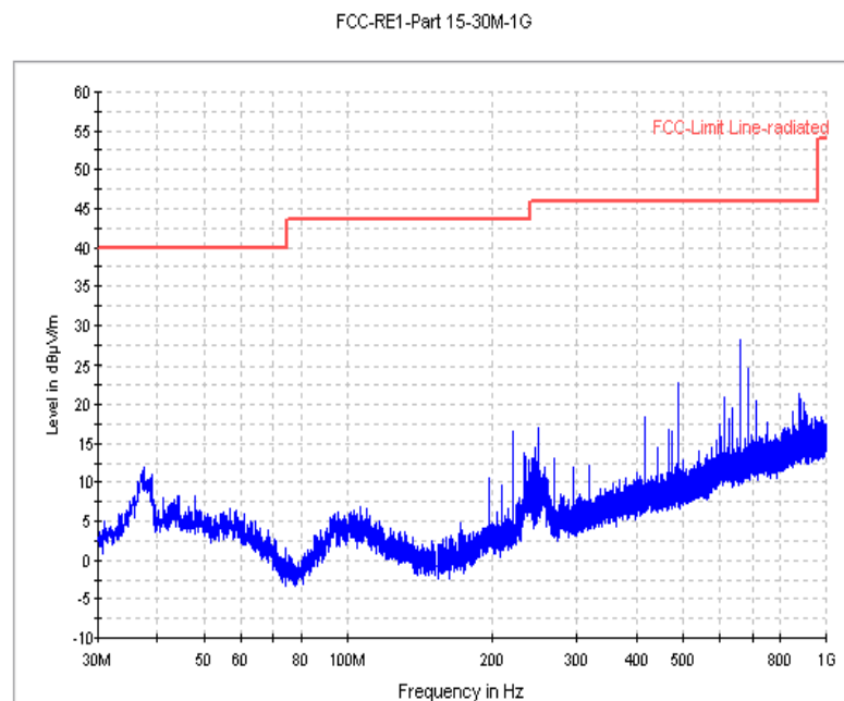
Fig. 59 Radiated Spurious Emission (802.11b, Ch11, 30MHz-1 GHz)
