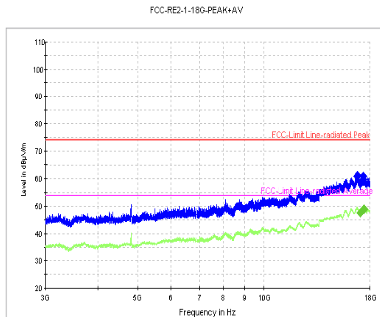
Fig. 66 Radiated Spurious Emission (802.11g, Ch1, 3 GHz-18 GHz)
