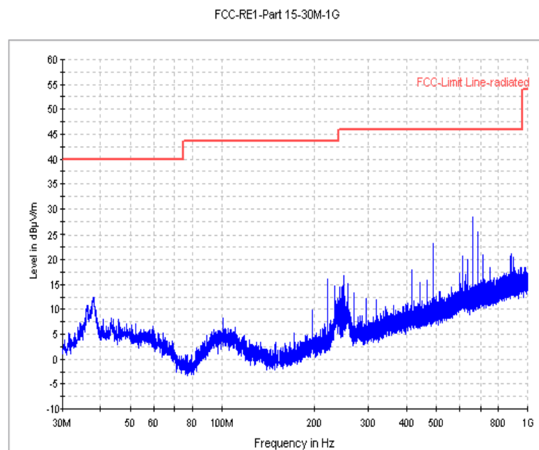
Fig. 56 Radiated Spurious Emission (802.11b, Ch6, 30MHz-1 GHz)
