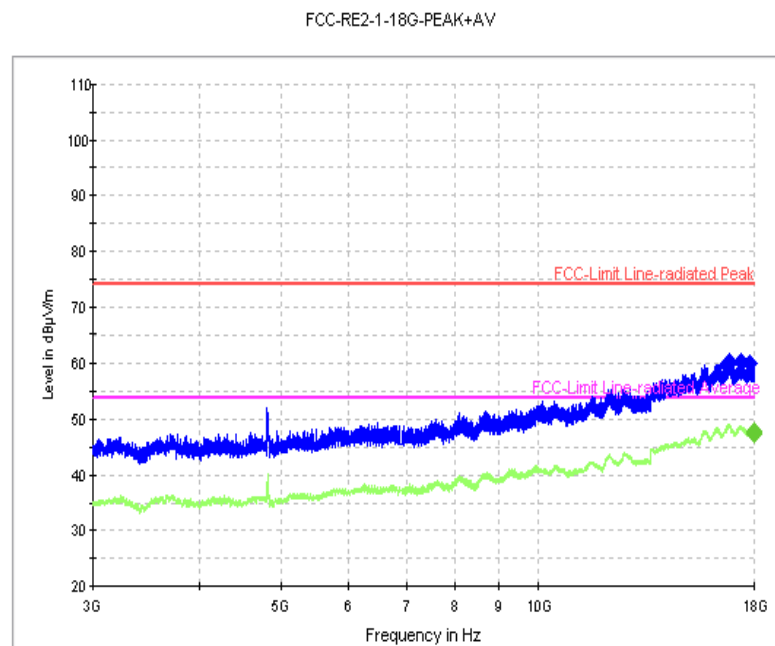
Fig. 69 Radiated Spurious Emission (802.11g, Ch6, 3 GHz-18 GHz)
