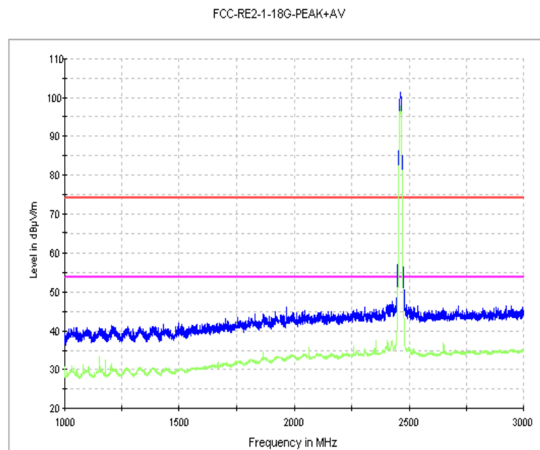
Fig. 57 Radiated Spurious Emission (802.11b, Ch6, 1 GHz-3 GHz)
