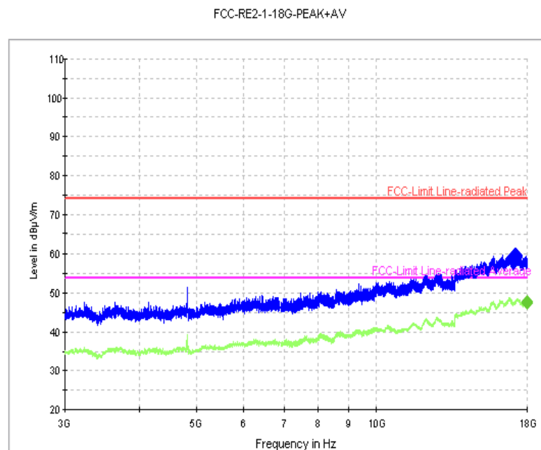
Fig. 77 Radiated Spurious Emission (802.11n-20M, Ch1, 3 GHz-18 GHz)
