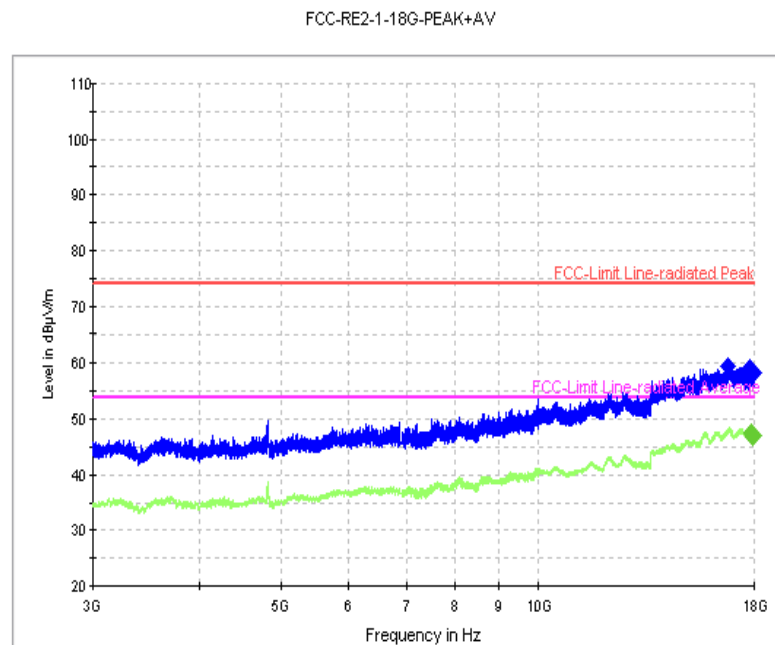
Fig. 80 Radiated Spurious Emission (802.11n-20M, Ch6, 3 GHz-18 GHz)
