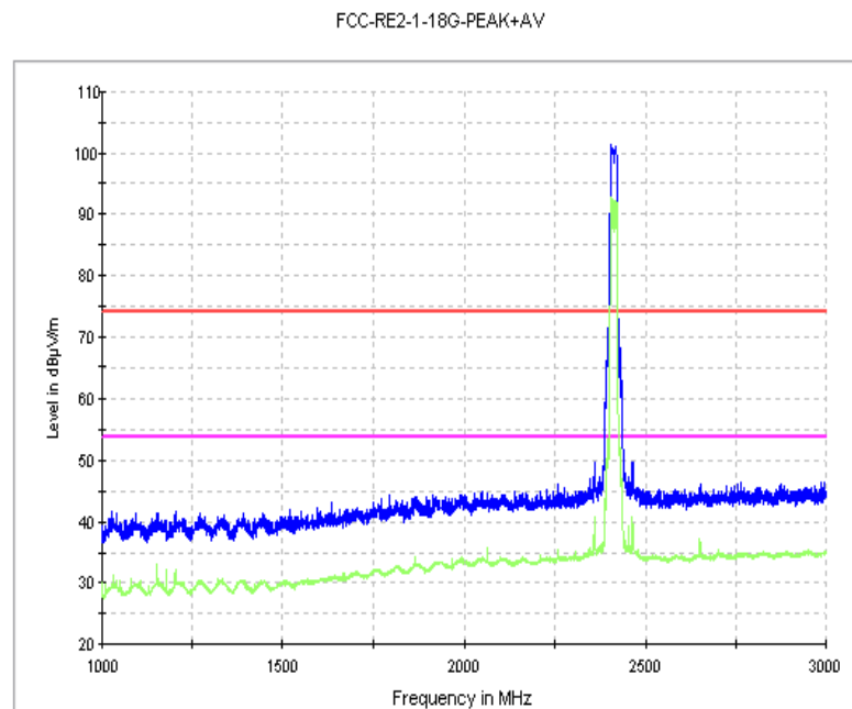
Fig. 76 Radiated Spurious Emission (802.11n-20M, Ch1, 1 GHz-3 GHz)
