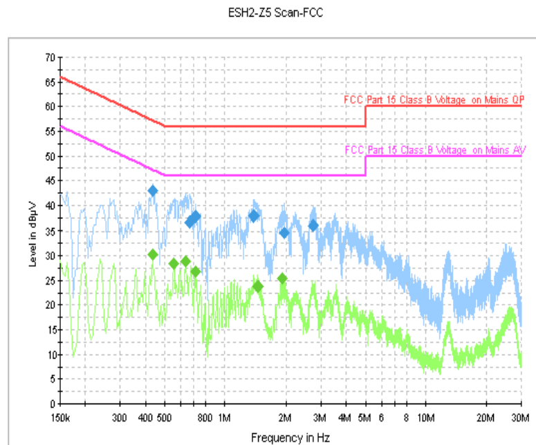
Fig. 89 AC Powerline Conducted Emission (Traffic, AE3)
