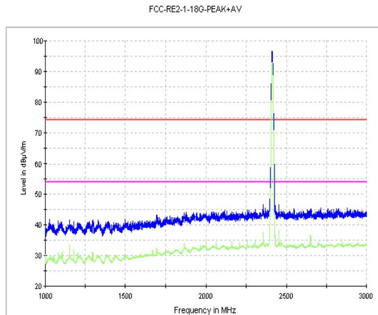
Fig. 54 Radiated Spurious Emission (802.11b, Ch1, 1 GHz-3 GHz)
