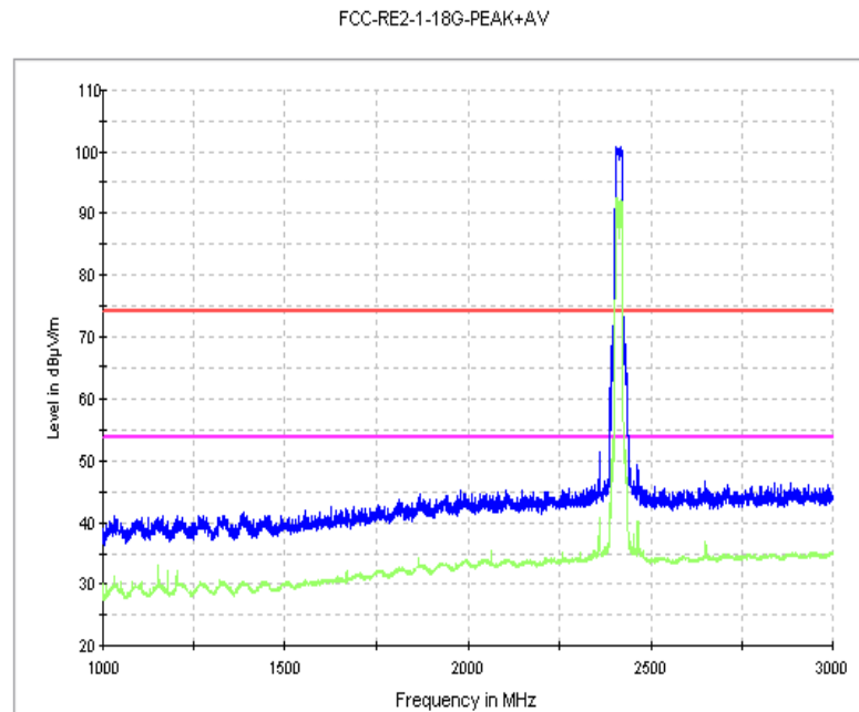
Fig. 79 Radiated Spurious Emission (802.11n-20M, Ch6, 1 GHz-3 GHz)
