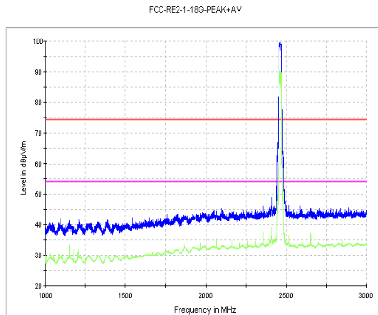
Fig. 71 Radiated Spurious Emission (802.11g, Ch11, 1 GHz-3 GHz)
