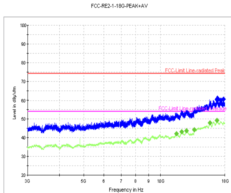
Fig. 55 Radiated Spurious Emission (802.11b, Ch1, 3 GHz-18 GHz)
