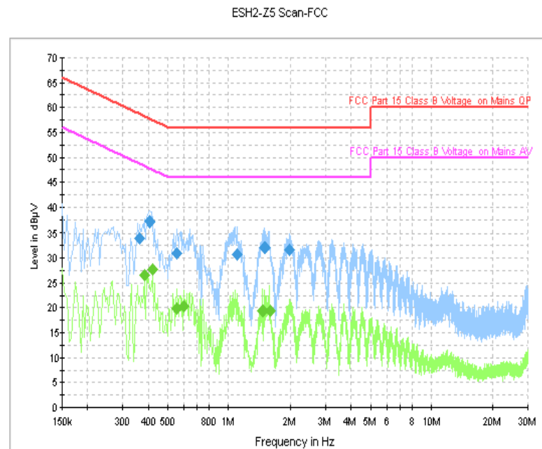
Fig. 88 AC Powerline Conducted Emission (Idle, AE2)
