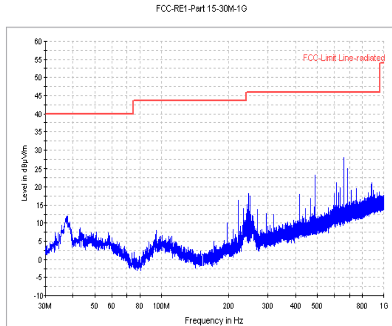
Fig. 75 Radiated Spurious Emission (802.11n-20M, Ch1, 30MHz-1 GHz)
