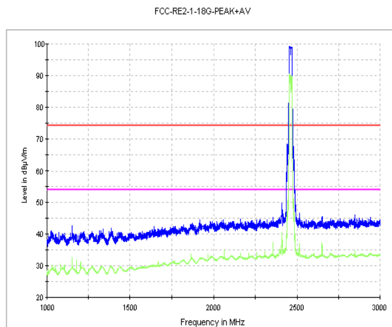
Fig. 82 Radiated Spurious Emission (802.11n-20M, Ch11, 1 GHz-3 GHz)
