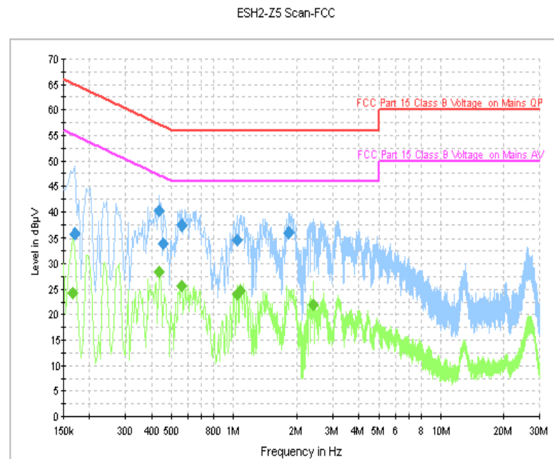
Fig. 90 AC Powerline Conducted Emission (Idle, AE3)
