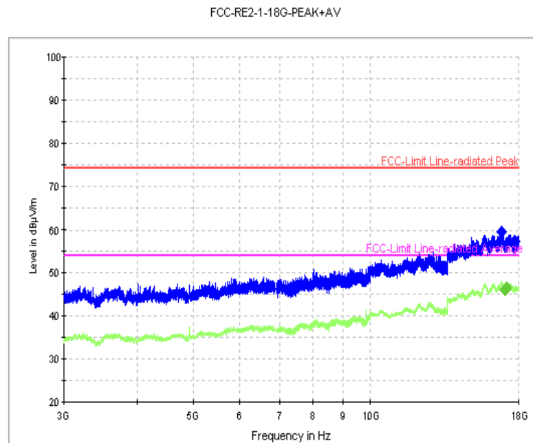
Fig. 83 Radiated Spurious Emission (802.11n-20M, Ch11, 3 GHz-18 GHz)
