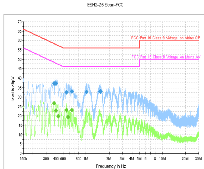
Fig. 87 AC Powerline Conducted Emission (Traffic, AE2)
