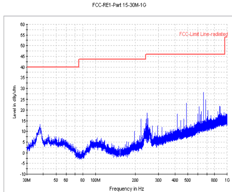
Fig. 53 Radiated Spurious Emission (802.11b, Ch1, 30MHz-1 GHz)
