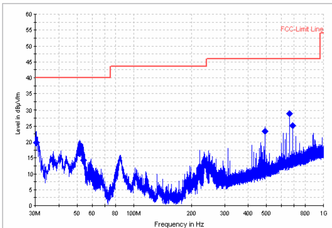
Figure A.3 Radiated Emission from 30MHz to 1GHz (Set.1, Charging mode)
