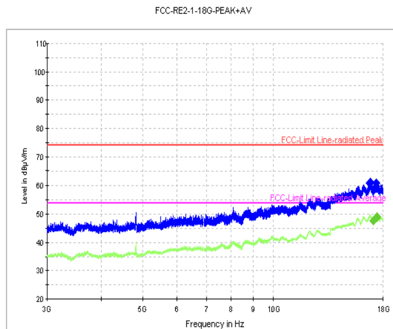
Fig. 66 Radiated Spurious Emission (802.11g, Ch1, 3 GHz-18 GHz)
