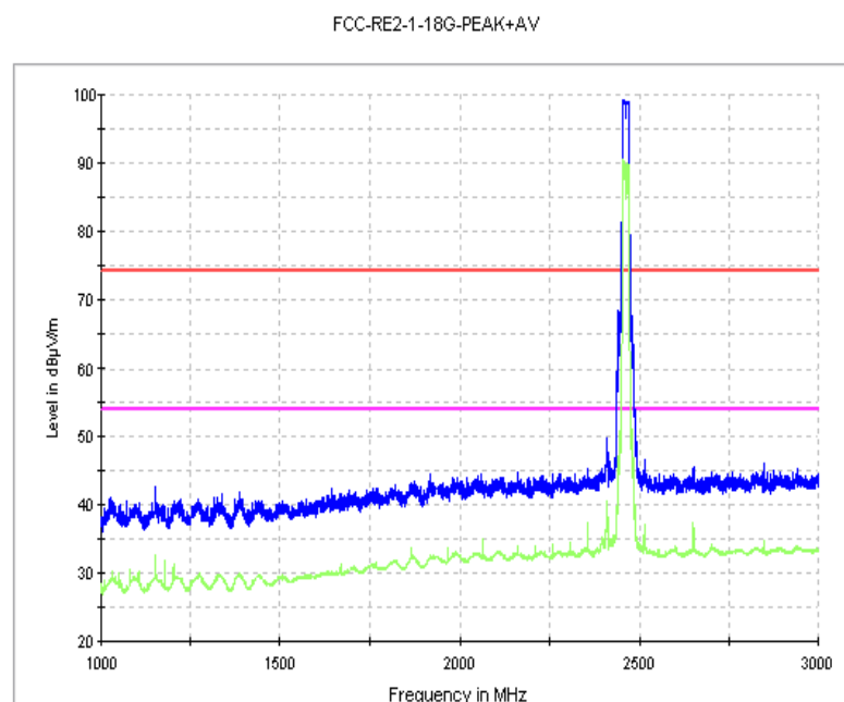
Fig. 82 Radiated Spurious Emission (802.11n-20M, Ch11, 1 GHz-3 GHz)
