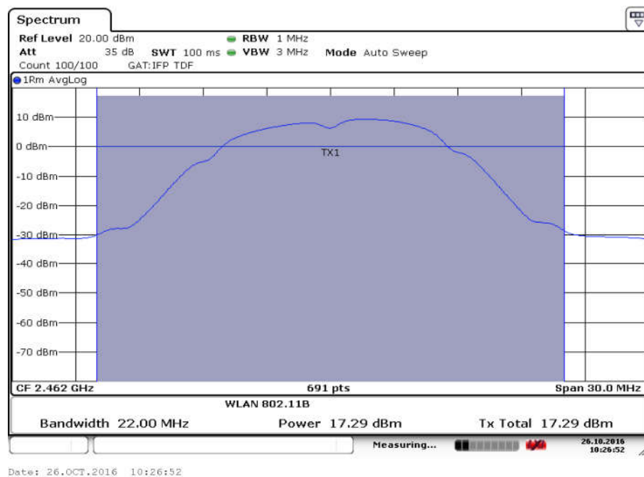
Fig.3 Maximum Average Output Power (802.11b, Ch 11,1Mbps)
