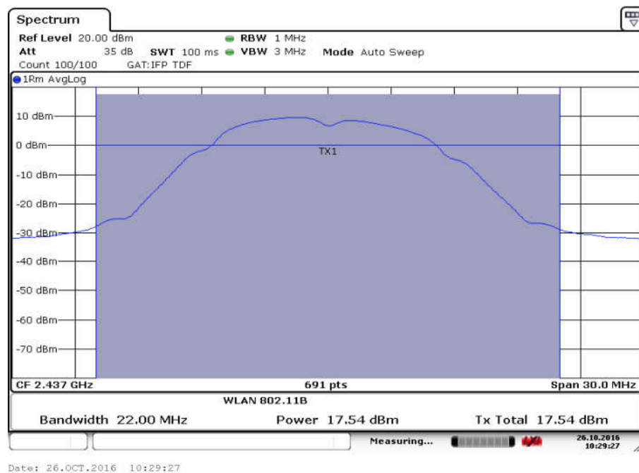
Fig.5 Maximum Average Output Power (802.11b, Ch 6,2Mbps)
