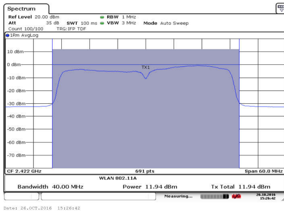
Fig.67 Maximum Average Output Power (802.11n-40MHz, Ch 3,MCS2)
