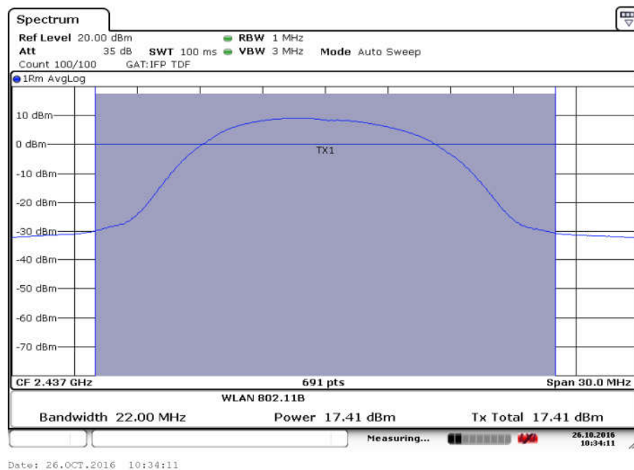
Fig.11 Maximum Average Output Power (802.11b, Ch 6,11Mbps)
