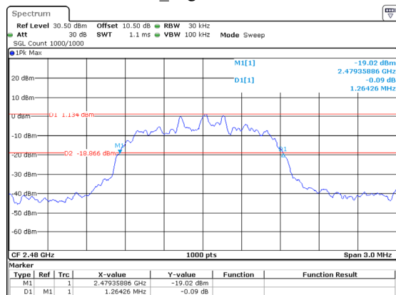
2DH1_High 1.264MHz
