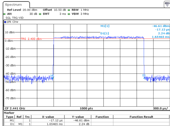
3DH3_Hop_2441 1.655ms
