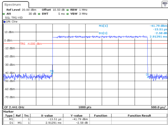
3DH5_Hop_2441 2.913ms
