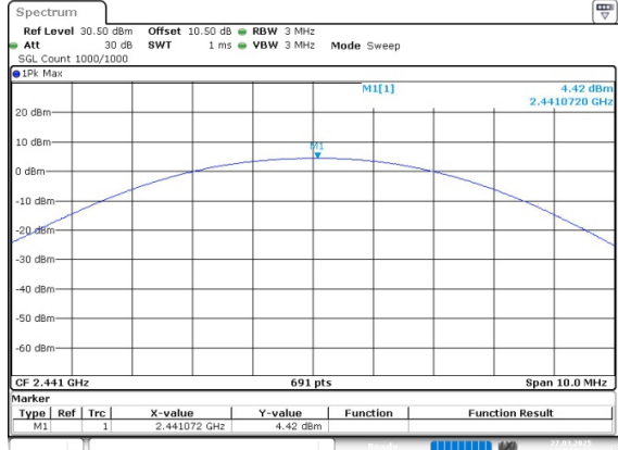
DH1_Middle 4.42dBm
