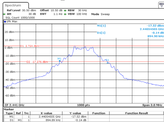
DH1_Middle 0.895MHz
