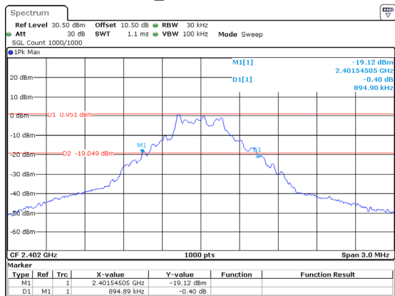
DH1_Low 0.895MHz
