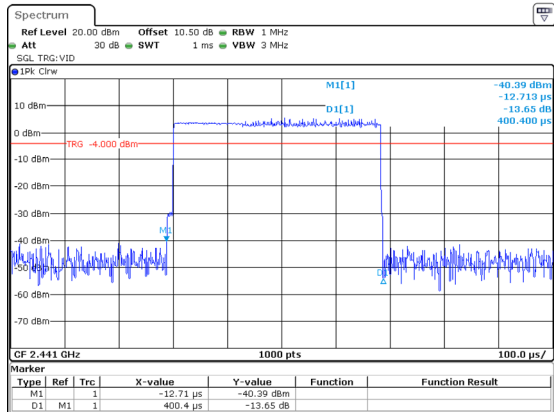
3DH1_Hop_2441 0.400ms
