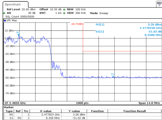
3DH1_Hopping_Upper
