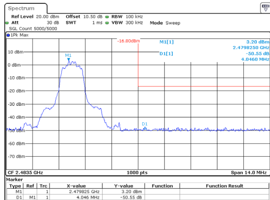
3DH1_High
