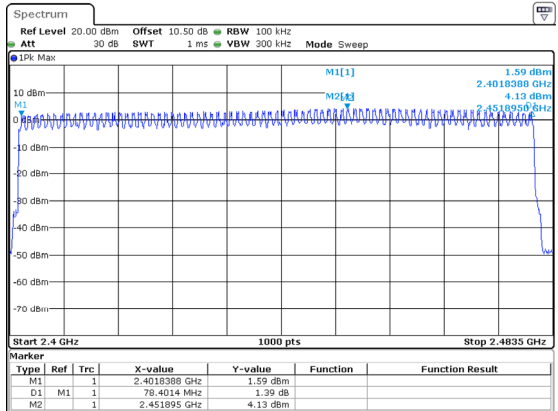
2DH1_Hopping 79
