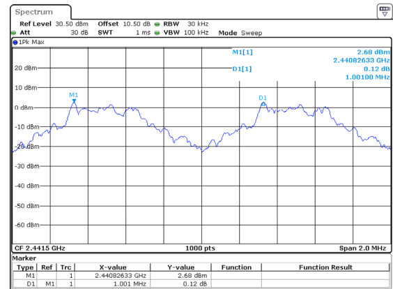
DH1_Middle 1.001MHz
