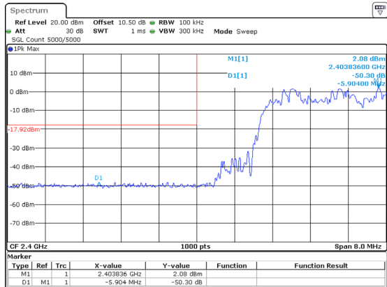
3DH1_Hopping_Lower
