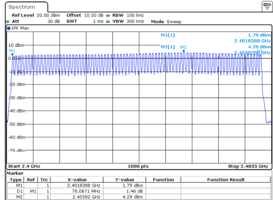
DH1_Hopping 79
