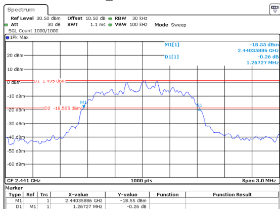
2DH1_Middle 1.267MHz
