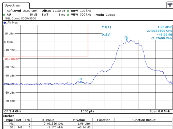
3DH1_Low
