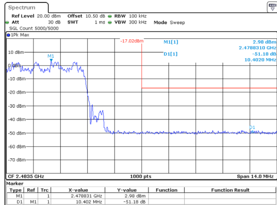
2DH1_Hopping_Upper
