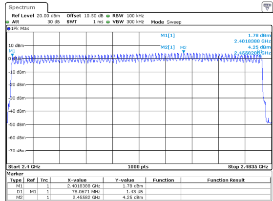
3DH1_Hopping 79
