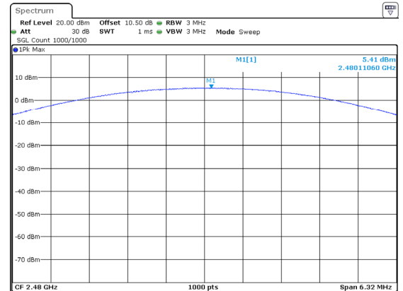
2DH1_High 5.41dBm
