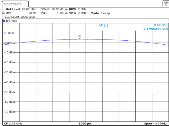
DH1_High 3.63dBm
