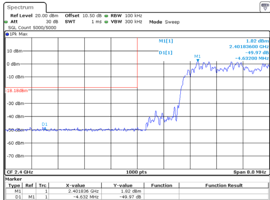
2DH1_Hopping_Lower
