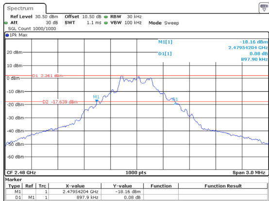
DH1_High 0.898MHz
