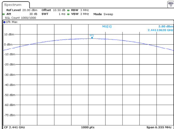
2DH1_Middle 5.80dBm
