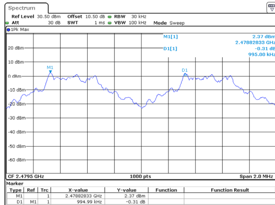
DH1_High 0.995MHz
