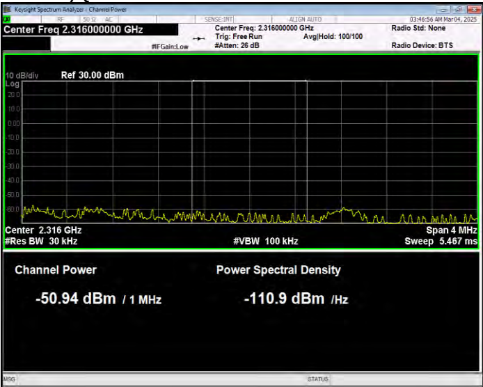
Band40(2305-2315) QPSK BW=5MHz Channel=38775 RB Size=1 Position=#0 Extended
