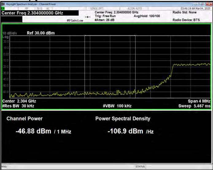
Band40(2305-2315) QPSK BW=5MHz Channel=38725 RB Size=25 Position=#0 Normal
