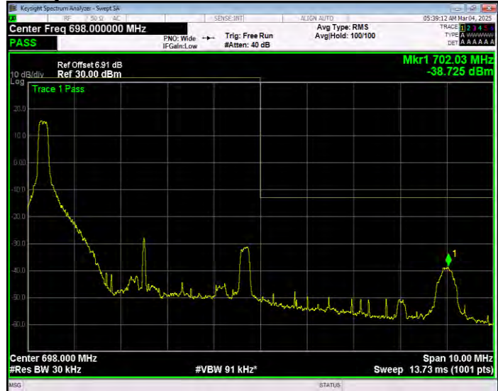
Band71 QPSK BW=5MHz Channel=133447 RB Size=1 Position=#Max Extended
