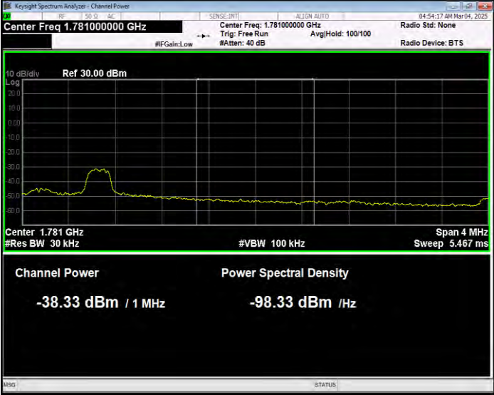
Band66 16QAM BW=5MHz Channel=132647 RB Size=1 Position=#Max Extended
