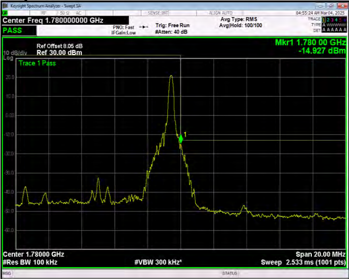
Band66 QPSK BW=10MHz Channel=132622 RB Size=50 Position=#0 Normal
