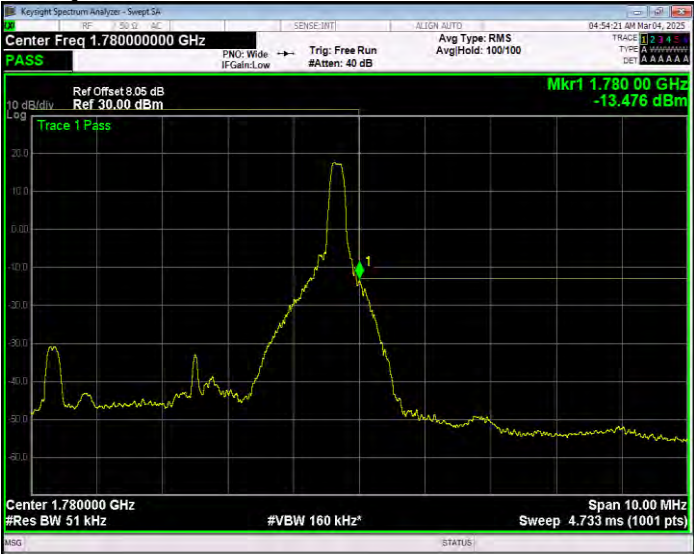
Band66 16QAM BW=5MHz Channel=132647 RB Size=25 Position=#0 Extended
