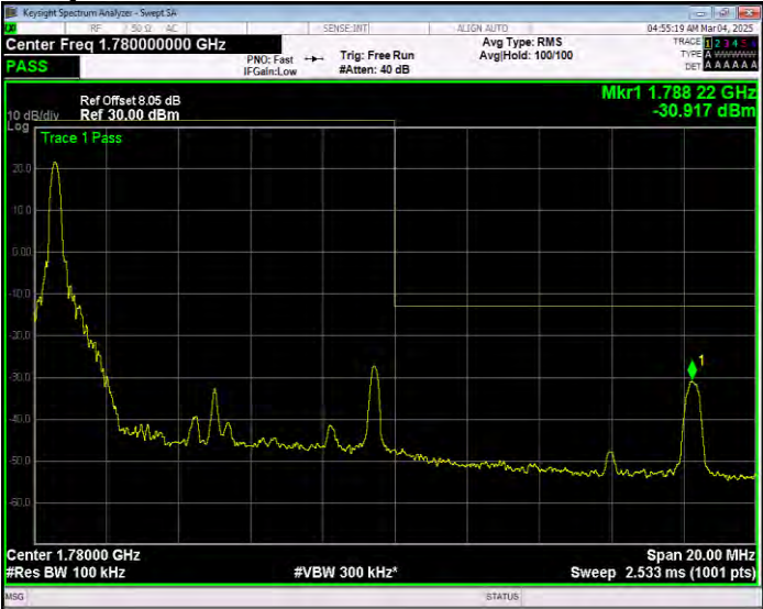
Band66 QPSK BW=10MHz Channel=132622 RB Size=1 Position=#0 Extended
