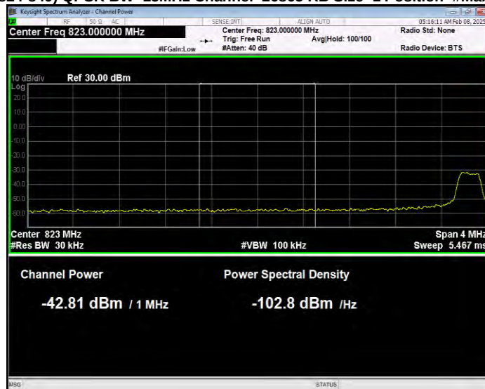
Band26(824-849) QPSK BW=15MHz Channel=26865 RB Size=1 Position=#Max Normal
