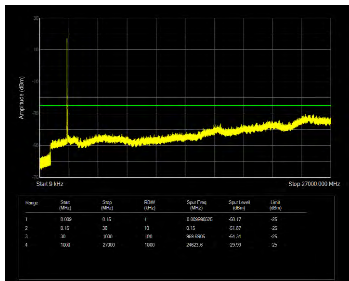
Band41(2535-2655) 16QAM BW=15MHz Channel=40640 RB Size=75 Position=#0
