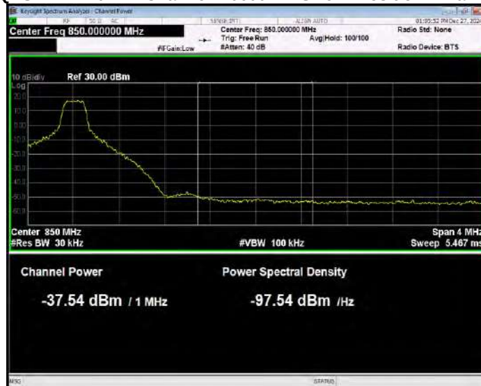
Band5 QPSK BW=10MHz Channel=20600 RB Size=1 Position=#Max Normal
