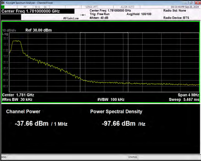
Band66 16QAM BW=15MHz Channel=132597 RB Size=1 Position=#Max Normal
