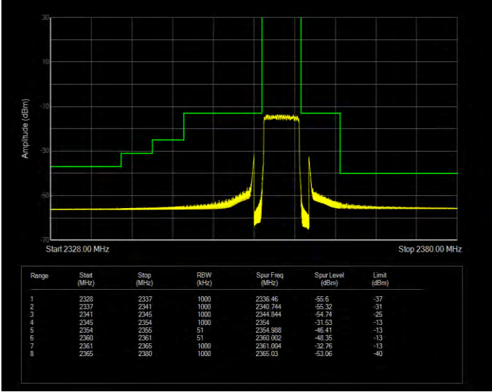
Band40(2350-2360) QPSK BW=10MHz Channel=39200 RB Size=1 Position=#0 Extended
