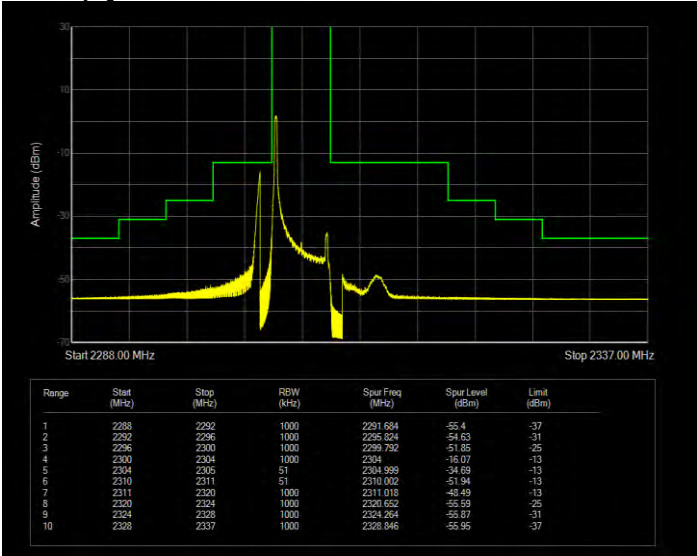
Band40(2305-2315) QPSK BW=5MHz Channel=38725 RB Size=25 Position=#0 Extended
