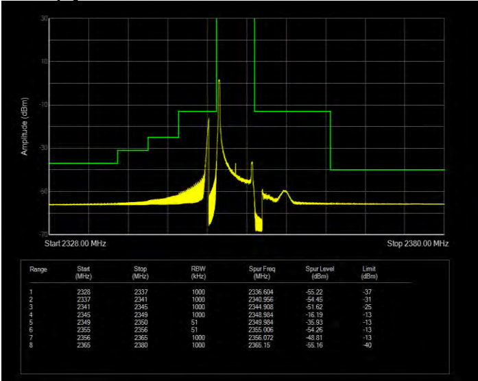
Band40(2350-2360) QPSK BW=5MHz Channel=39175 RB Size=25 Position=#0 Extended
