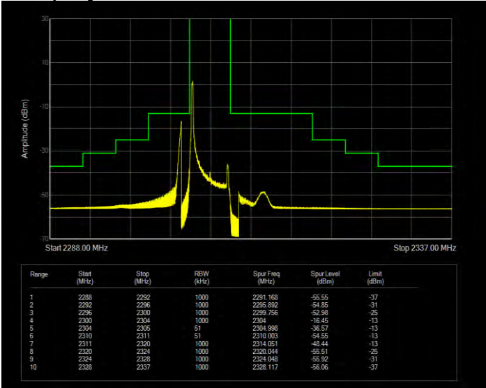
Band40(2305-2315) 16QAM BW=5MHz Channel=38725 RB Size=25 Position=#0 Extended
