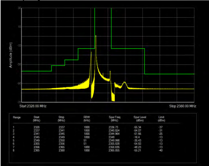
Band40(2350-2360) 16QAM BW=5MHz Channel=39175 RB Size=25 Position=#0 Extended
