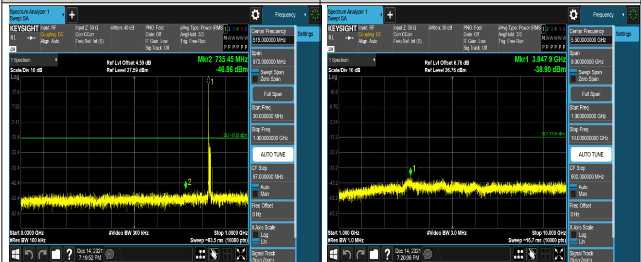
Band5-10MHz-16QAM-20450-1RB#0-Range1:30~1000MHz
