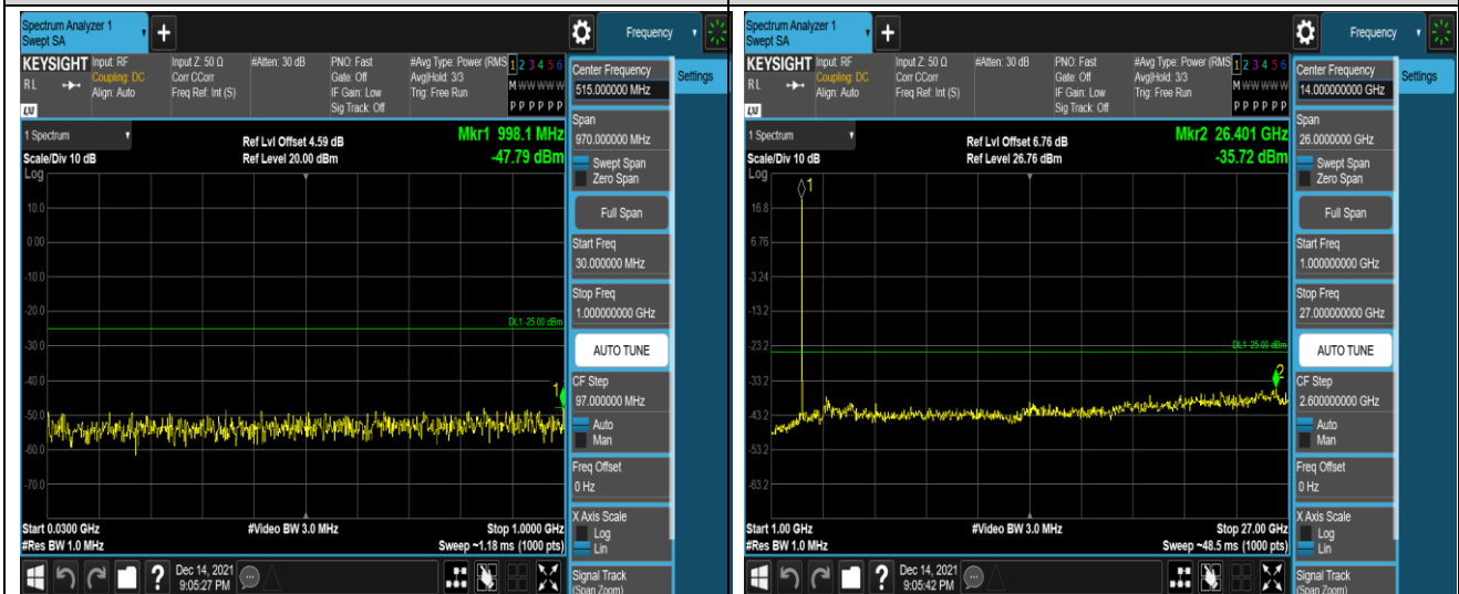
Band7-20MHz-QPSK-21100-1RB#0-Range1:30~1000MHz
