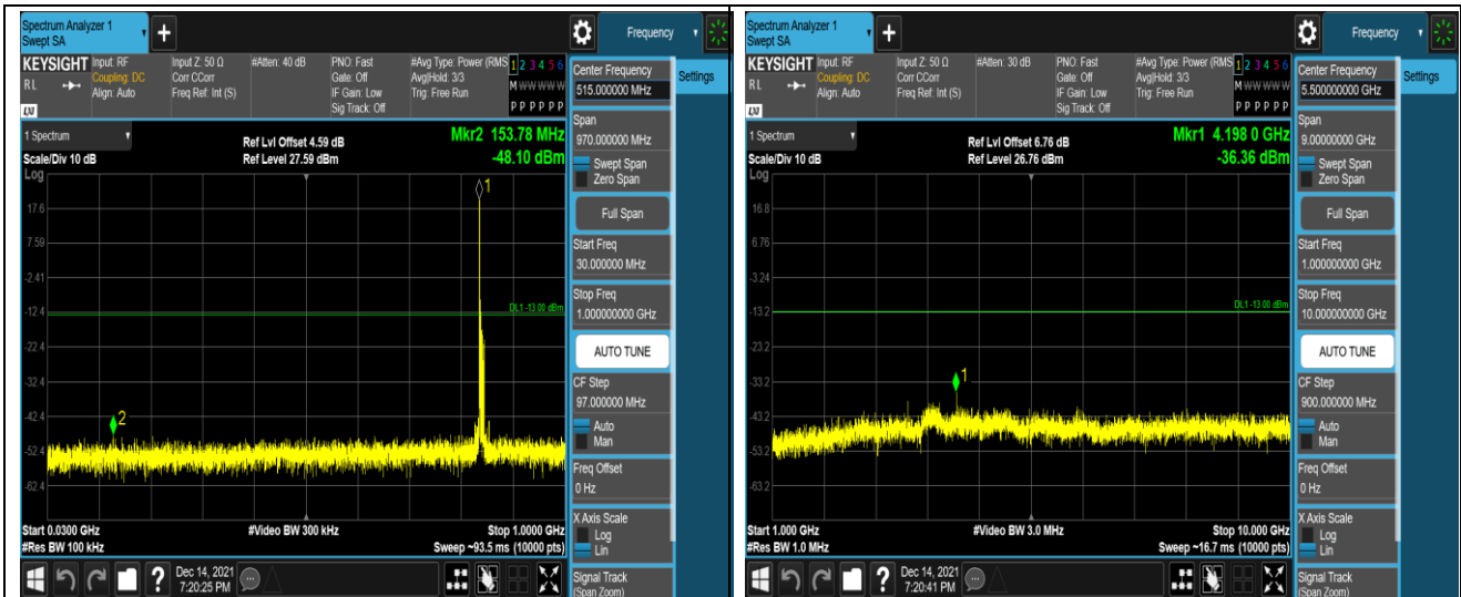
Band5-10MHz-QPSK-20600-1RB#0-Range1:30~1000MHz
