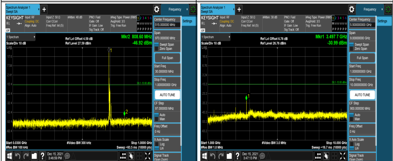
Band12-10MHz-QPSK-23060-1RB#0-Range1:30~1000MHz
