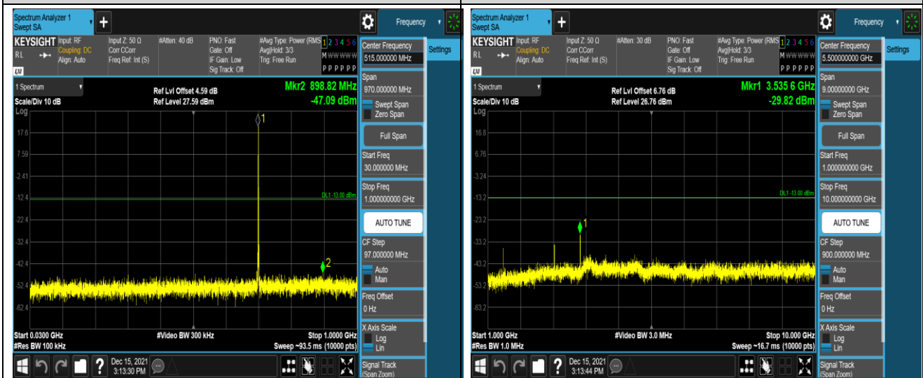
Band12-1.4MHz-QPSK-23095-1RB#0-Range1:30~1000MHz
