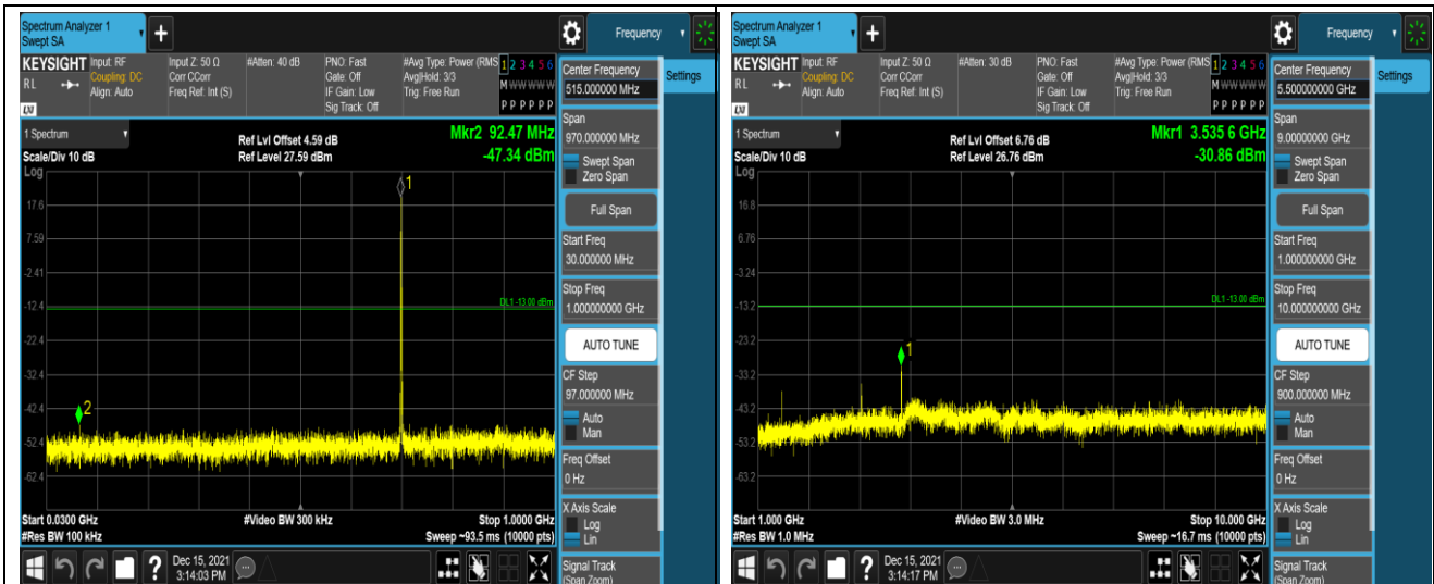
Band12-1.4MHz-16QAM-23173-1RB#0-Range1:30~1000MHz
