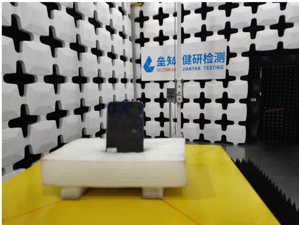
Above 1GHz
