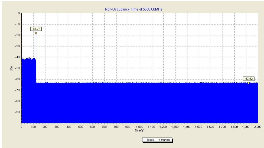
Fig.6 Non-Occupancy Period (HT80 Frequency Band: 5470MHz ~ 5725MHz)
