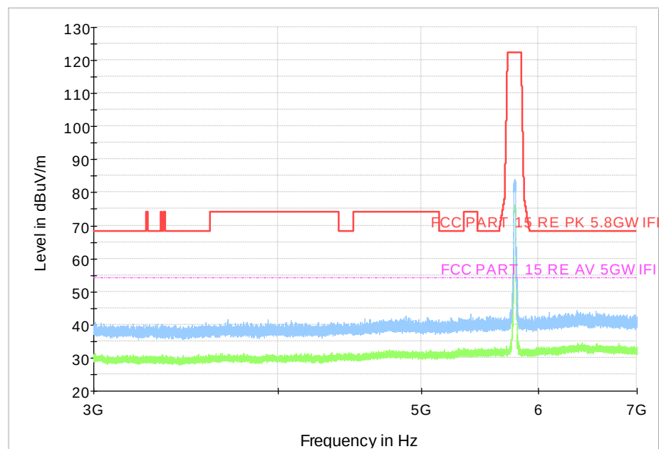
Fig. 121 Transmitter Spurious Emission (802.11a, CH157 5785MHz, 3 GHz-7 GHz)
