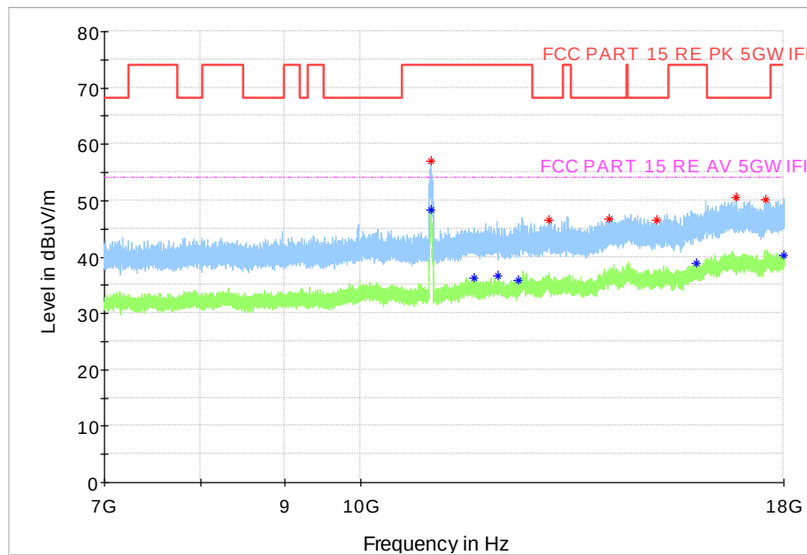
Fig. 176 Transmitter Spurious Emission (802.11n-HT40, CH102 5510MHz, 7 GHz-18 GHz)
