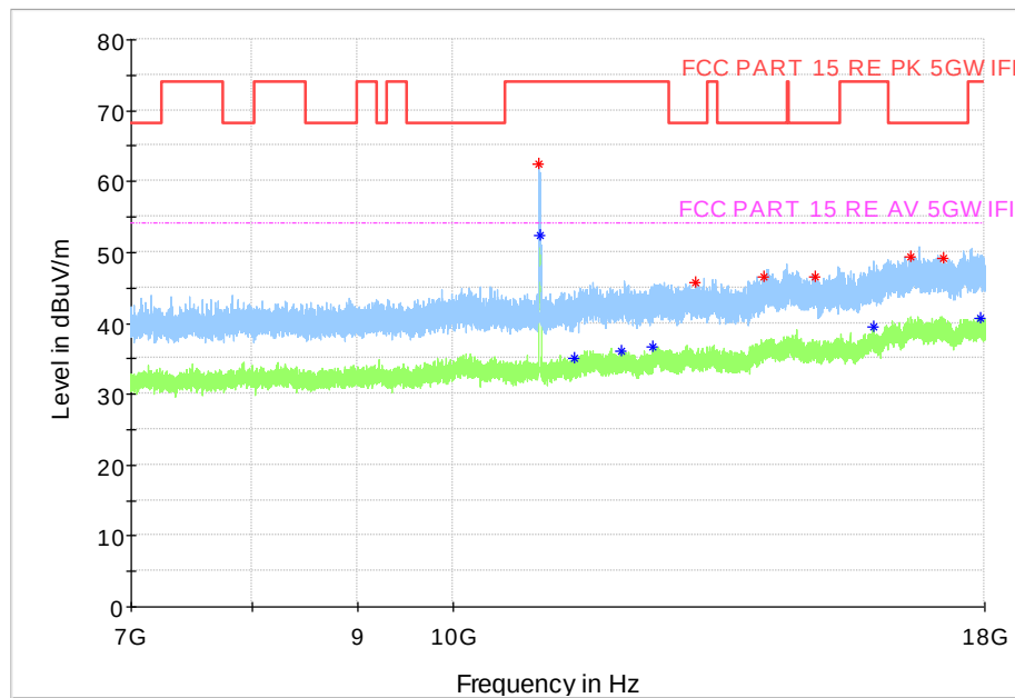
Fig. 146 Transmitter Spurious Emission (802.11n-HT20, CH100 5500MHz, 7 GHz-18 GHz)
