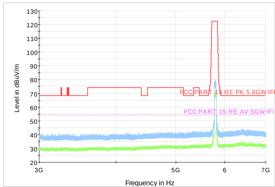
Fig. 187 Transmitter Spurious Emission (802.11n-HT40, CH159 5795MHz, 3 GHz-7 GHz)
