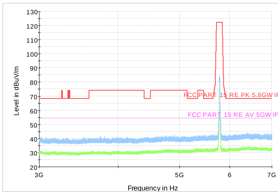
Fig. 157 Transmitter Spurious Emission (802.11n-HT20, CH157 5785MHz, 3 GHz-7 GHz)
