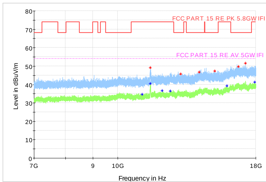
Fig. 119 Transmitter Spurious Emission (802. 11a, CH149 5745MHz, 7 GHz-18 GHz)
