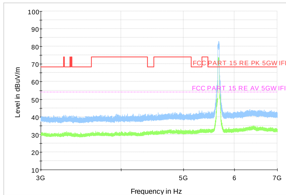
Fig. 181 Transmitter Spurious Emission (802.11n-HT40, CH134 5670MHz, 3 GHz-7 GHz)
