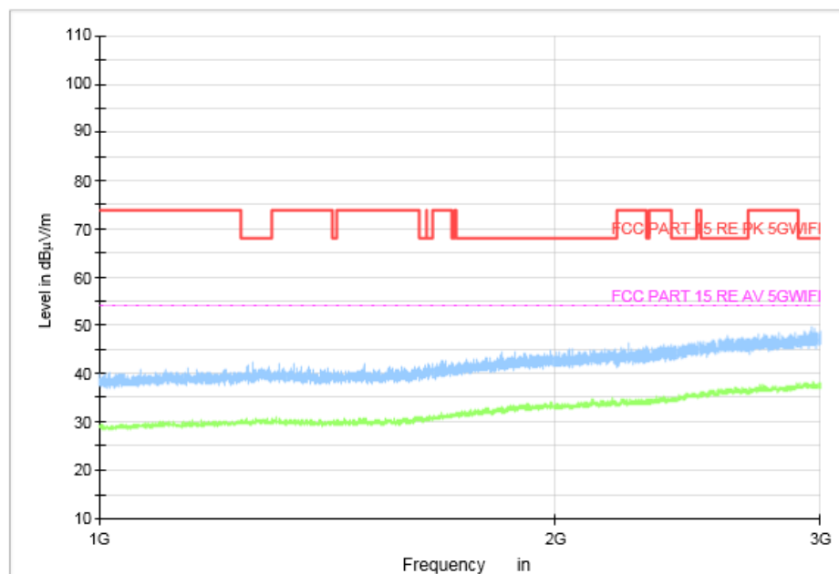
Fig. 183 Transmitter Spurious Emission (802.11n-HT40, CH151 5755MHz, 1 GHz-3 GHz)
