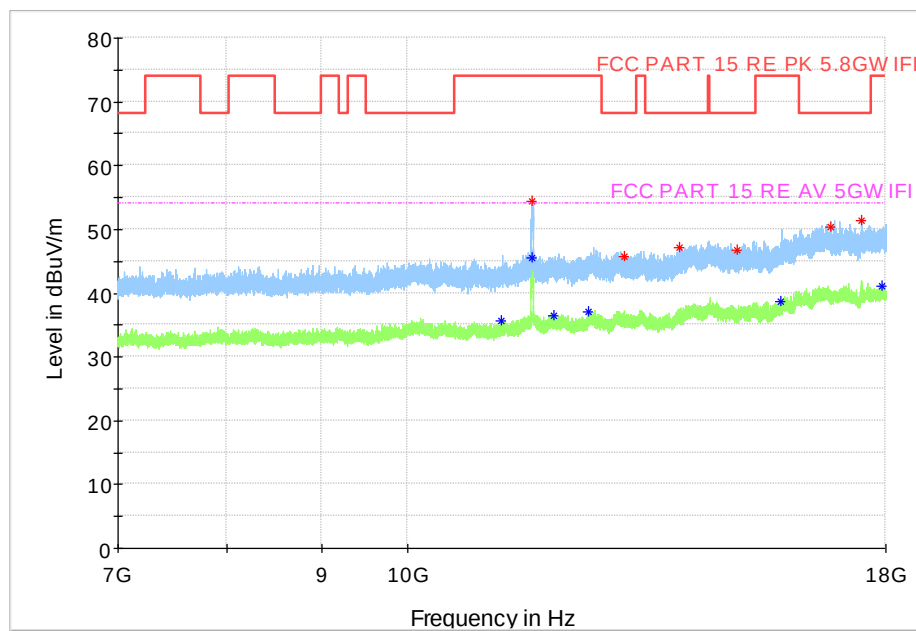
Fig. 161 Transmitter Spurious Emission (802.11n-HT20, CH165 5825MHz, 7 GHz-18 GHz)
