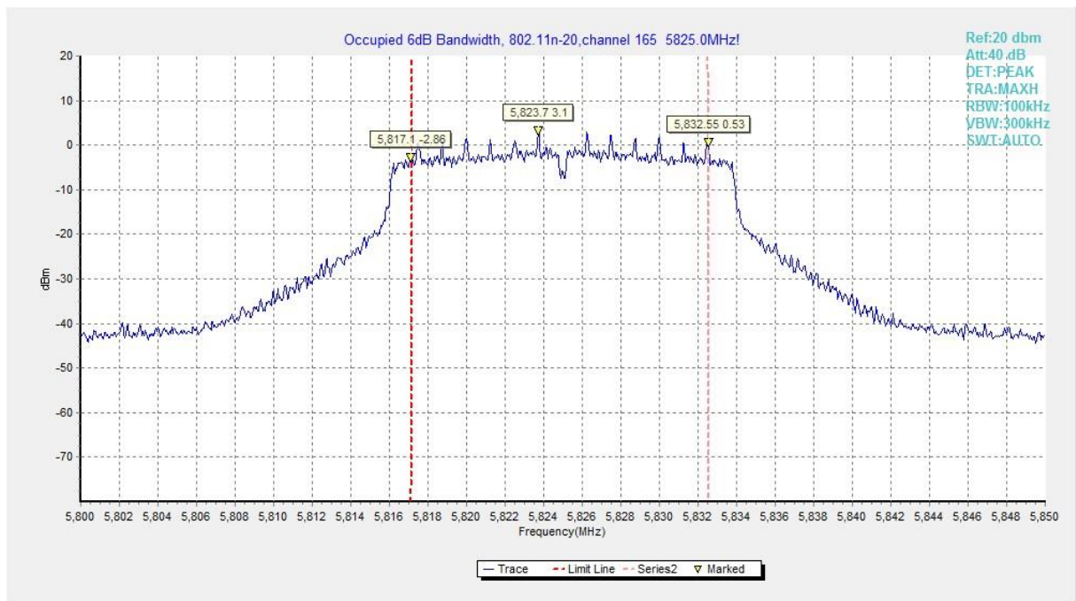
Fig. 35 Occupied 6dB Bandwidth (802.11n-HT20, 5825MHz)
