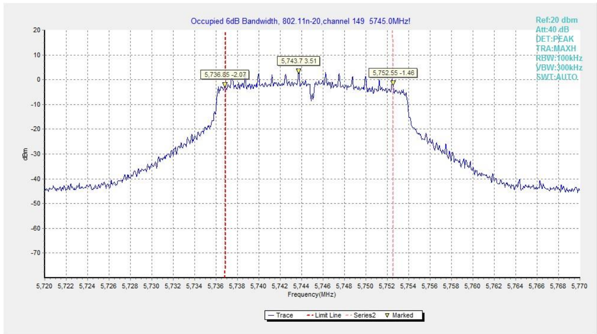
Fig. 33 Occupied 6dB Bandwidth (802.11n-HT20, 5745MHz)
