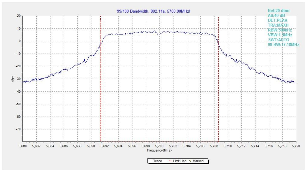
Fig. 47 99% Occupied Bandwidth (802. 11a, 5700MHz)
