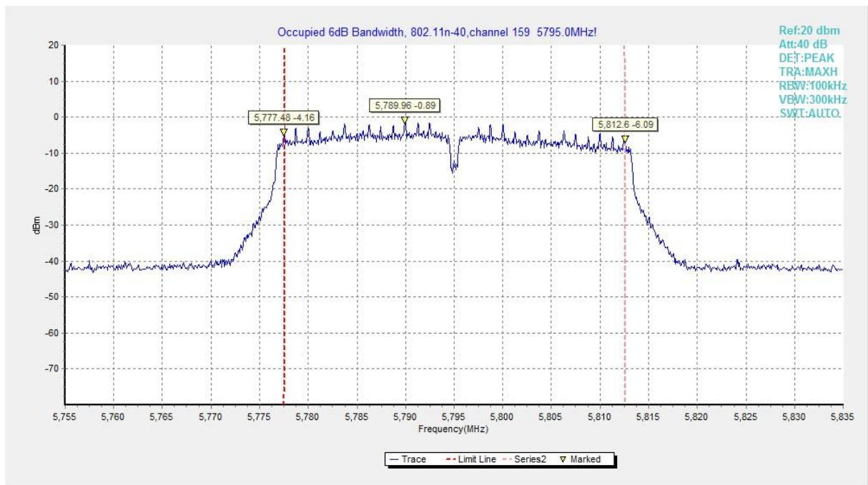
Fig. 37 Occupied 6dB Bandwidth (802.11n-HT40, 5795MHz)
