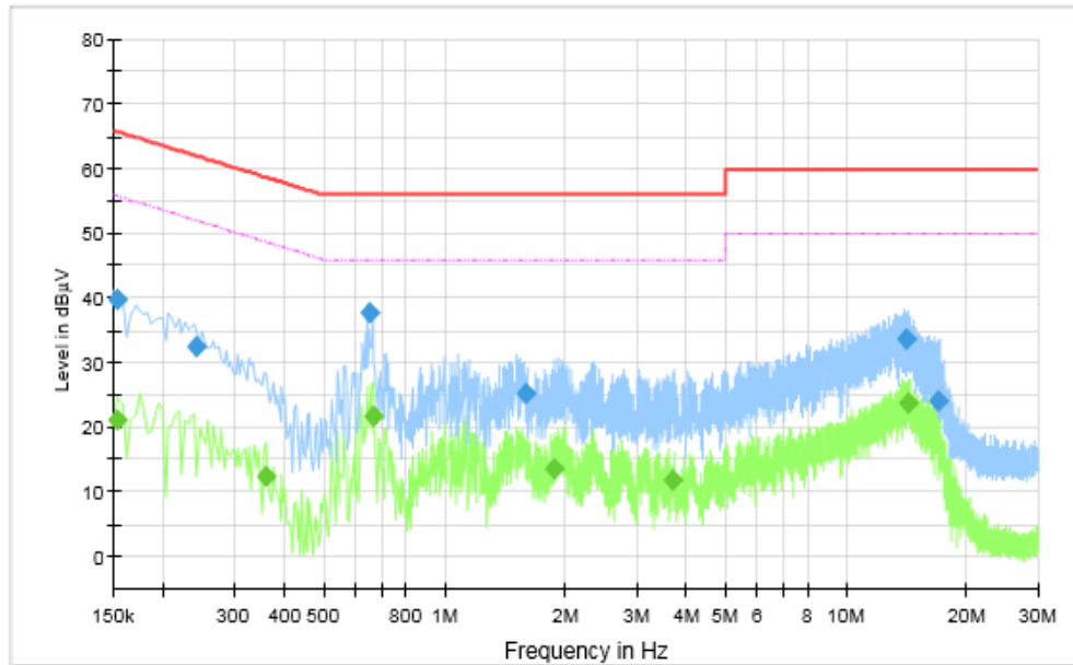
Fig.94 AC Power line Conducted Emission (Idle), LE 2M
