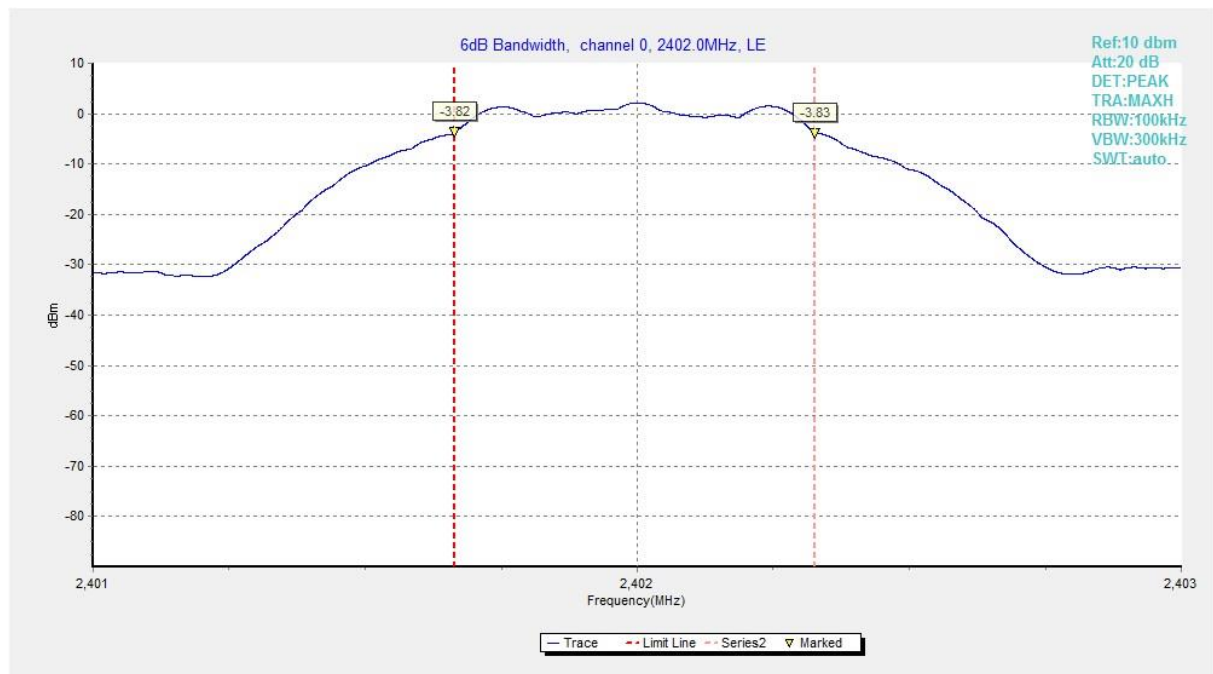
Fig.10 6dB Bandwidth (Ch 0), LE 1M
