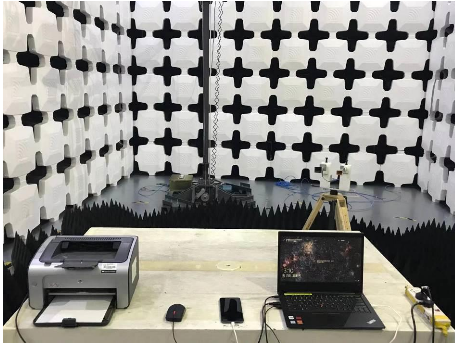
3. Radiated Emissions (Part 15B,Data transfer Mode)(18GHz-26.5GHz)
