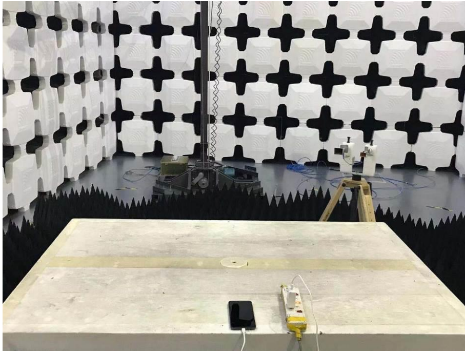
7. Radiated Emissions (Part 15B, Charging Mode) (18GHz-26.5GHz)
