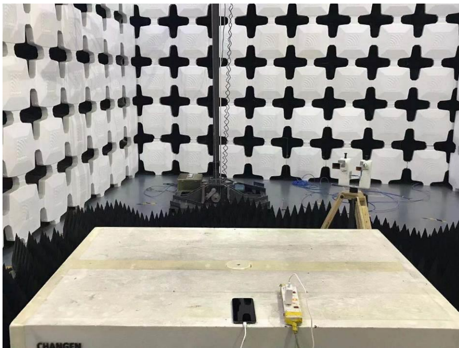
8. Radiated Emissions (Part 15B, Charging Mode) (26.5GHz-30GHz)
