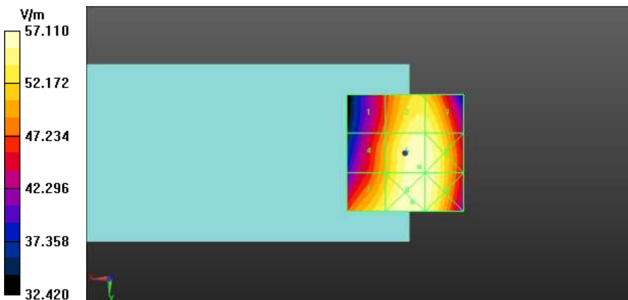
Fig A.7 HAC RF E-Field CDMA BC0
