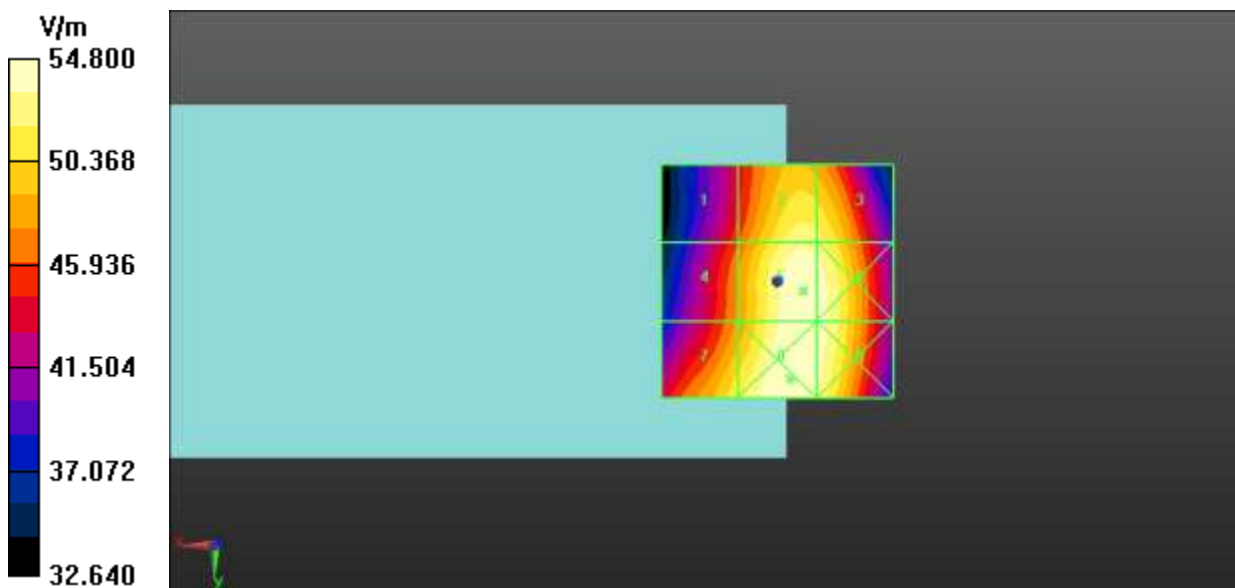
Fig A.9 HAC RF E-Field CDMA BC0
