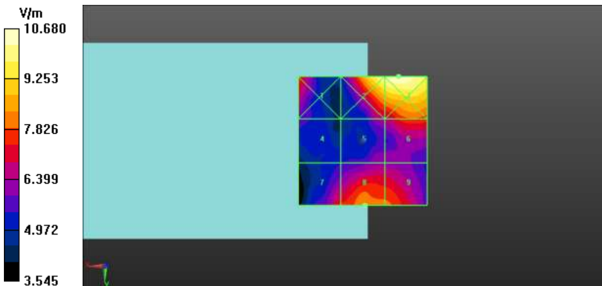
Fig A.16 HAC RF E-Field LTE-Band 41 High
