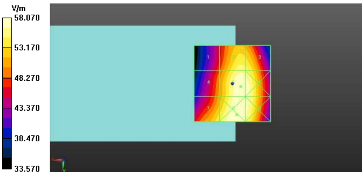
Fig A.8 HAC RF E-Field CDMA BC0
