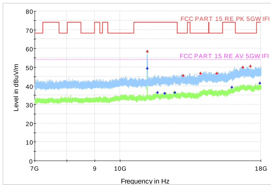
Fig. 113 Transmitter Spurious Emission (802. 11a, CH120 5600MHz, 7 GHz-18 GHz)
