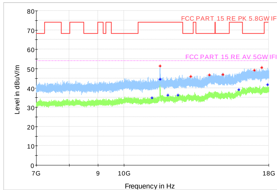
Fig. 122 Transmitter Spurious Emission (802. 11a, CH157 5785MHz, 7 GHz-18 GHz)
