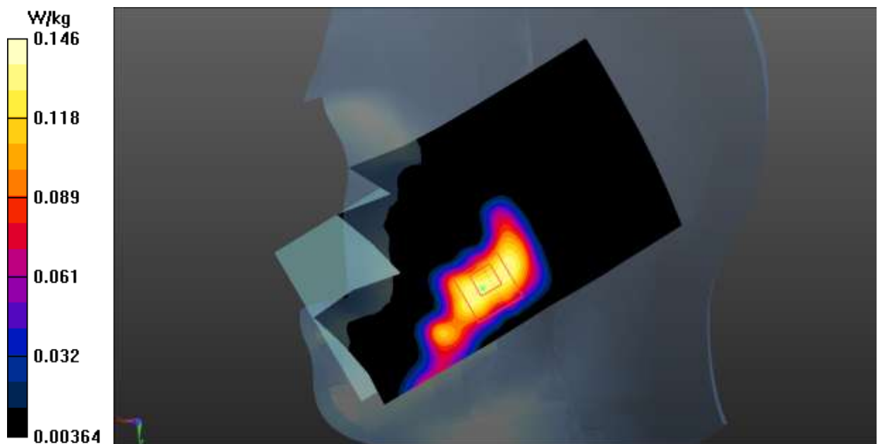
Fig.3 GSM 1900 Head
