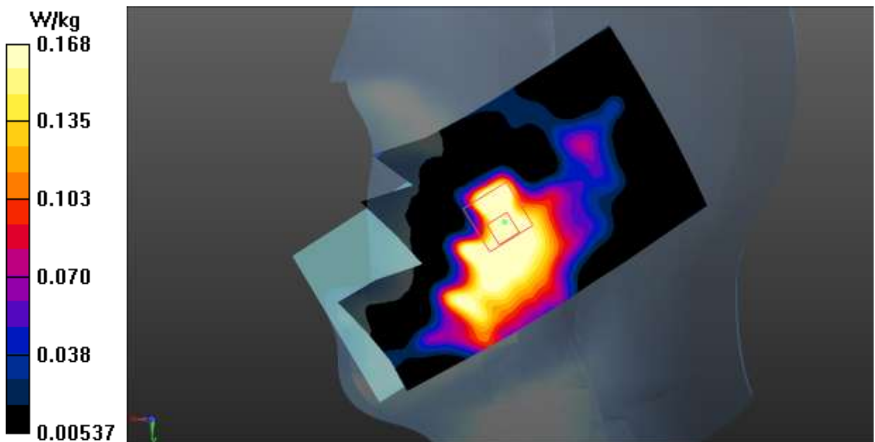
Fig.1 GSM 850 Head
