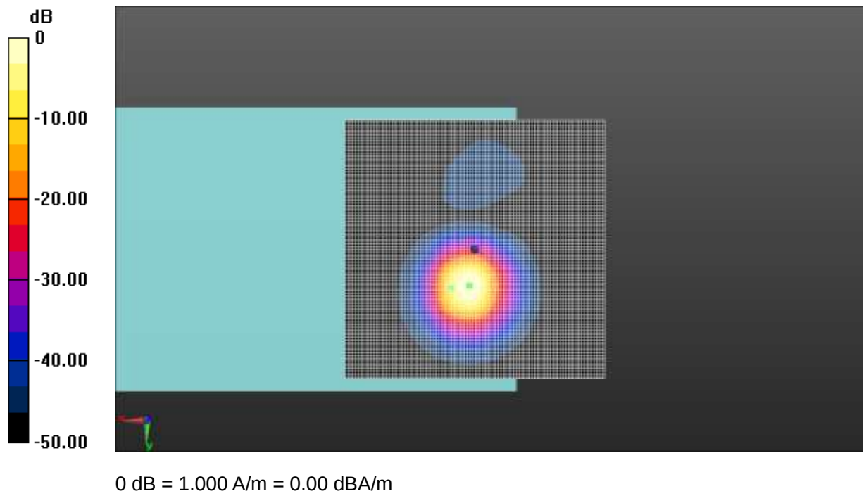
Fig A.26 T-Coil GSM 1900-Z
