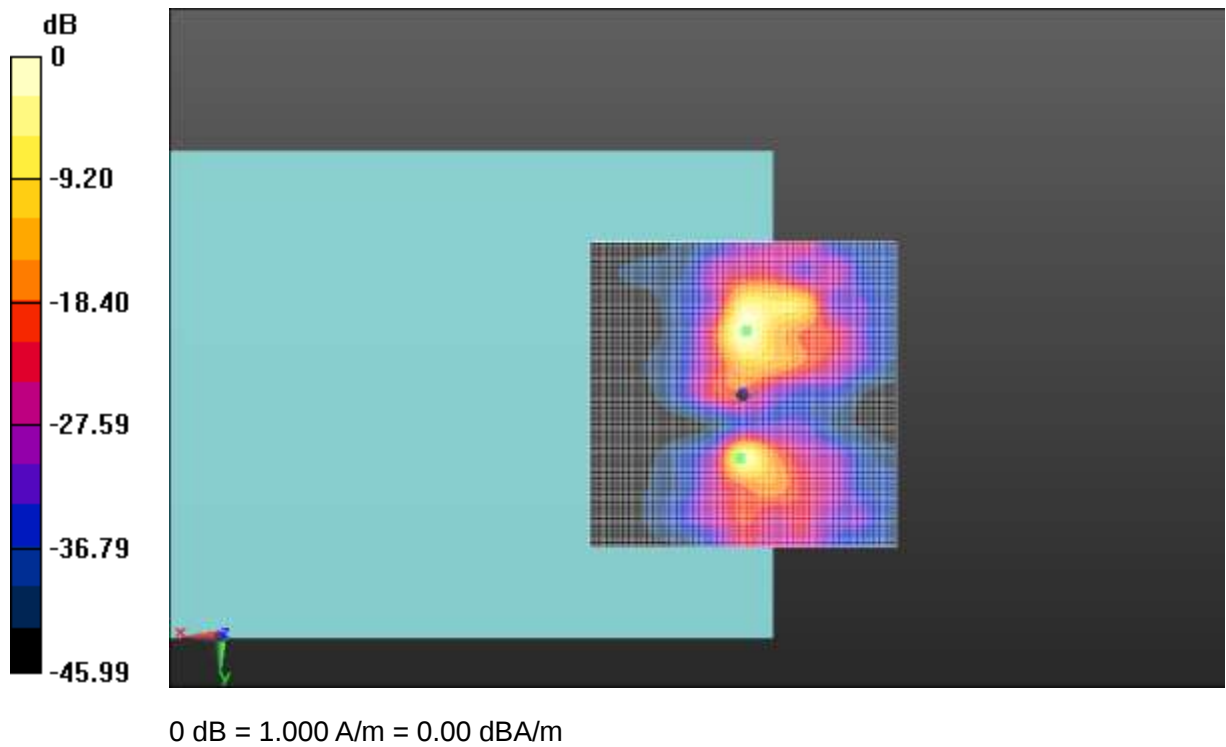
Fig A.18 T-Coil LTE-Band 71-Y
