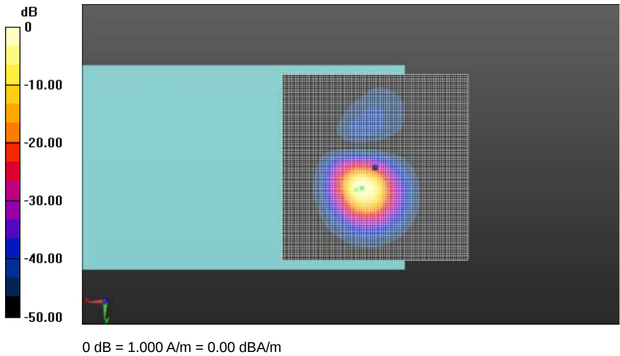
Fig A.28 T-Coil CDMA BC1-Z
