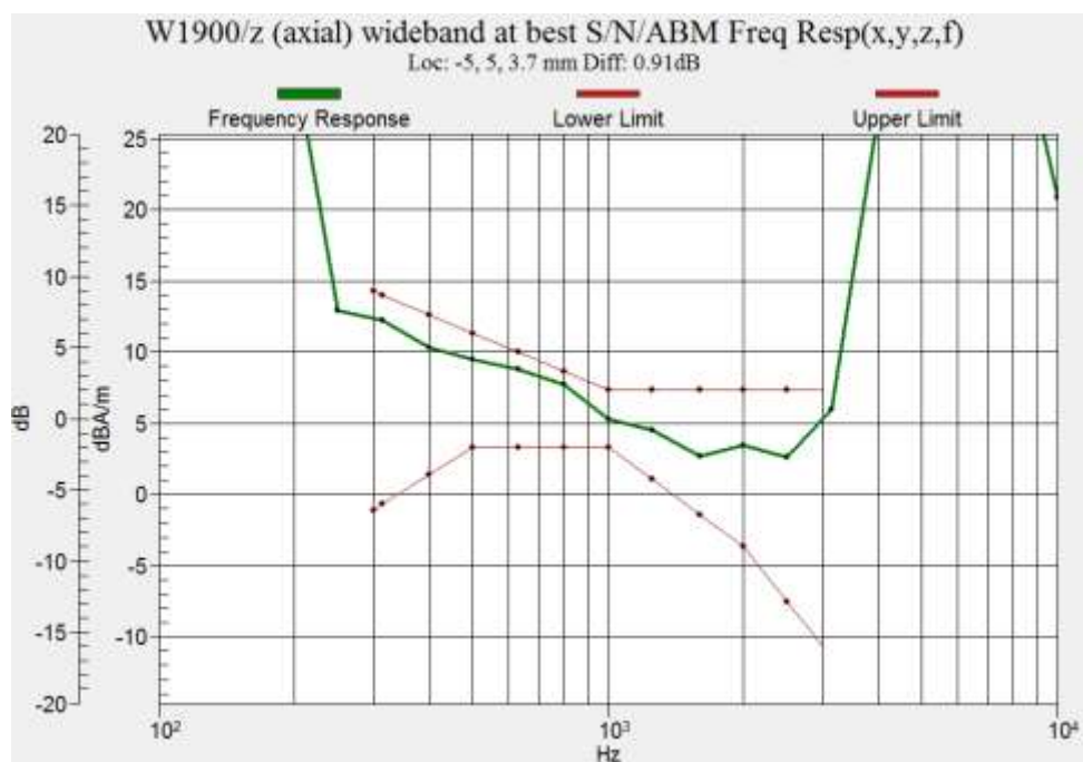
Figure B.30 Frequency Response of WCDMA Band 2 (Google Duo)
