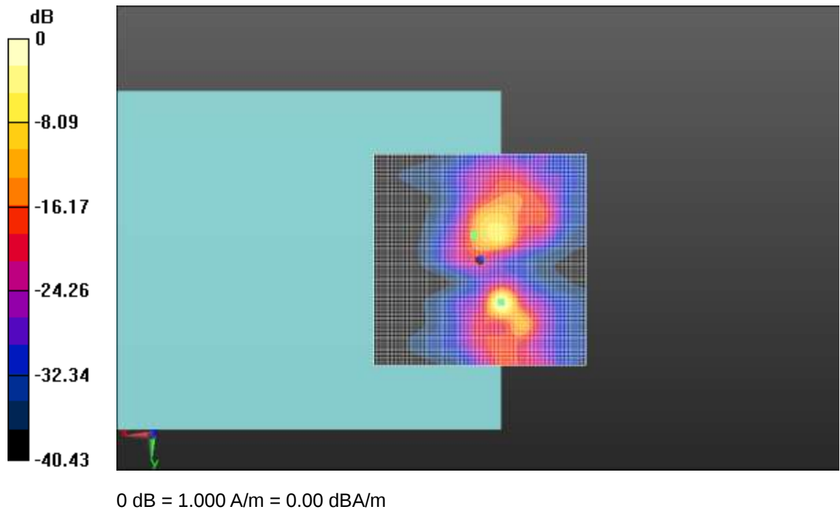
Fig A.14 T-Coil LTE-Band 13-Y
