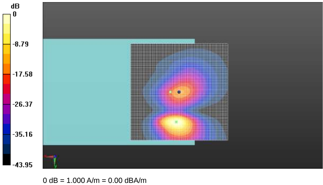
Fig A.31 T-Coil WCDMA Band 4-Y
