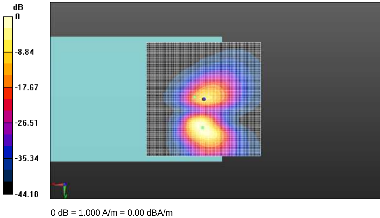
Fig A.32 T-Coil WCDMA Band 5-Y
