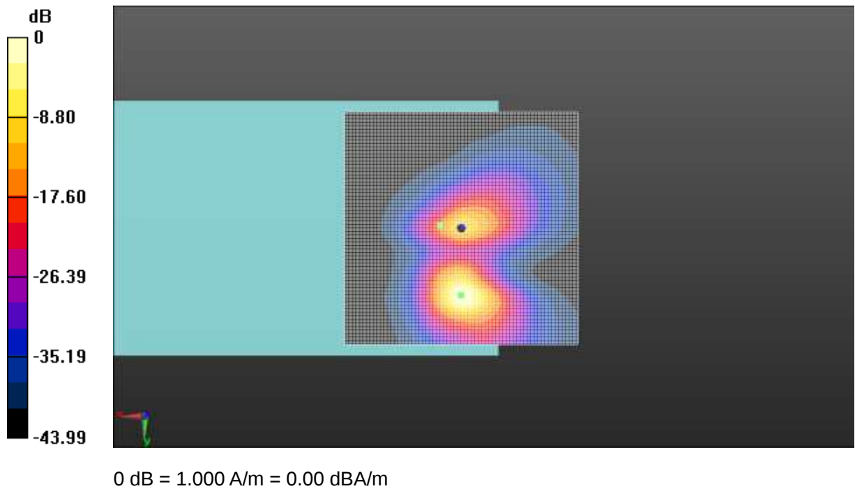
Fig A.30 T-Coil WCDMA Band 2-Y
