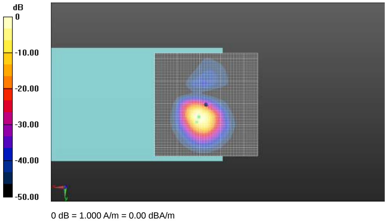
Fig A.27 T-Coil CDMA BC0-Z
