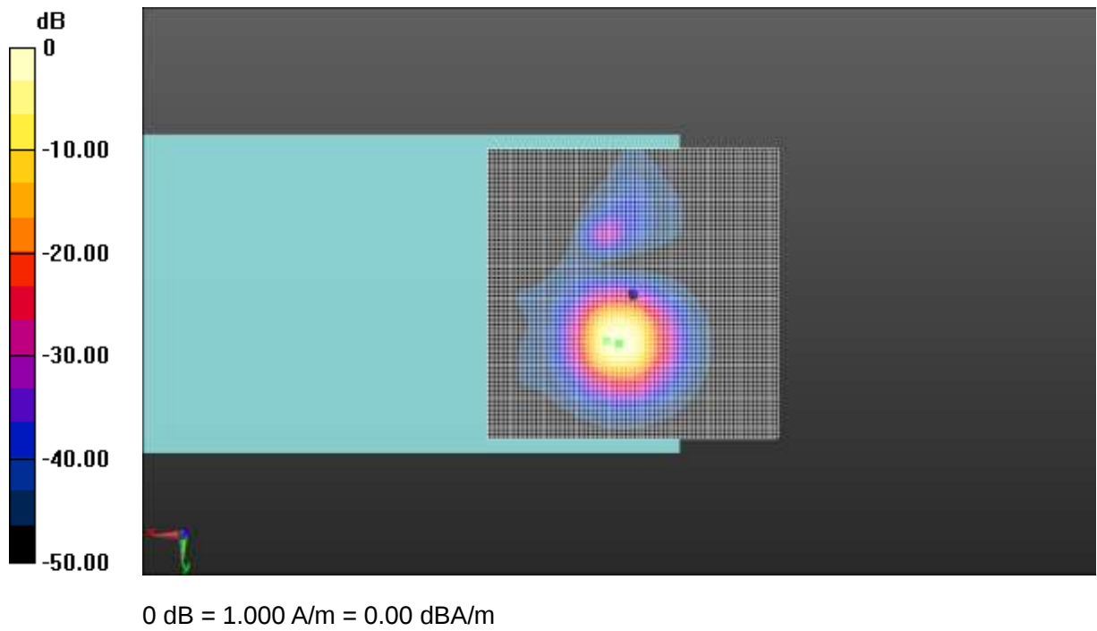
Fig A.33 T-Coil LTE-Band 41-Z
