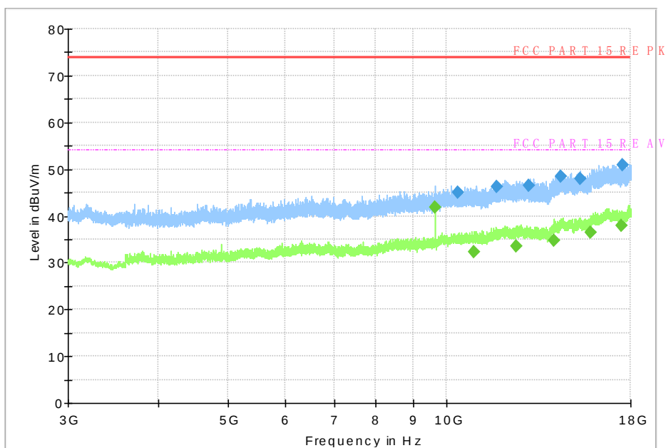
Fig. 54 Radiated Spurious Emission (GFSK, Ch39, 3 GHz ~18 GHz)
