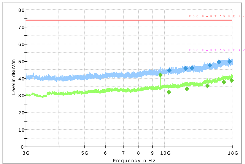
Fig. 68 Radiated Spurious Emission (8DPSK, Ch0, 3 GHz ~18 GHz)
