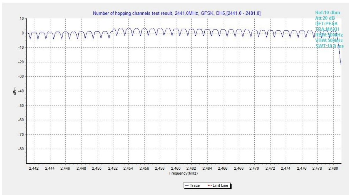
Fig. 94 Hopping channel ch39~78 (GFSK, Ch39)
