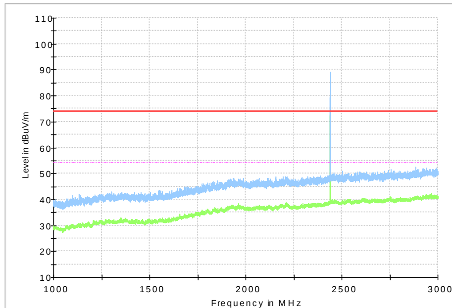
Fig. 69 Radiated Spurious Emission (8DPSK, Ch39, 1 GHz ~3 GHz)
