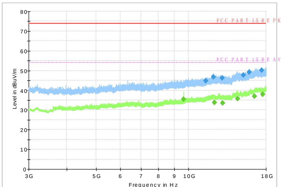
Fig. 52 Radiated Spurious Emission (GFSK, Ch0, 3 GHz ~18 GHz)
