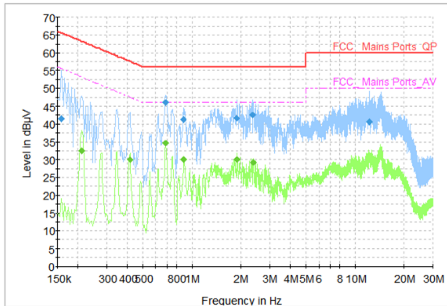
Fig. 102 AC Powerline Conducted Emission (Traffic)
