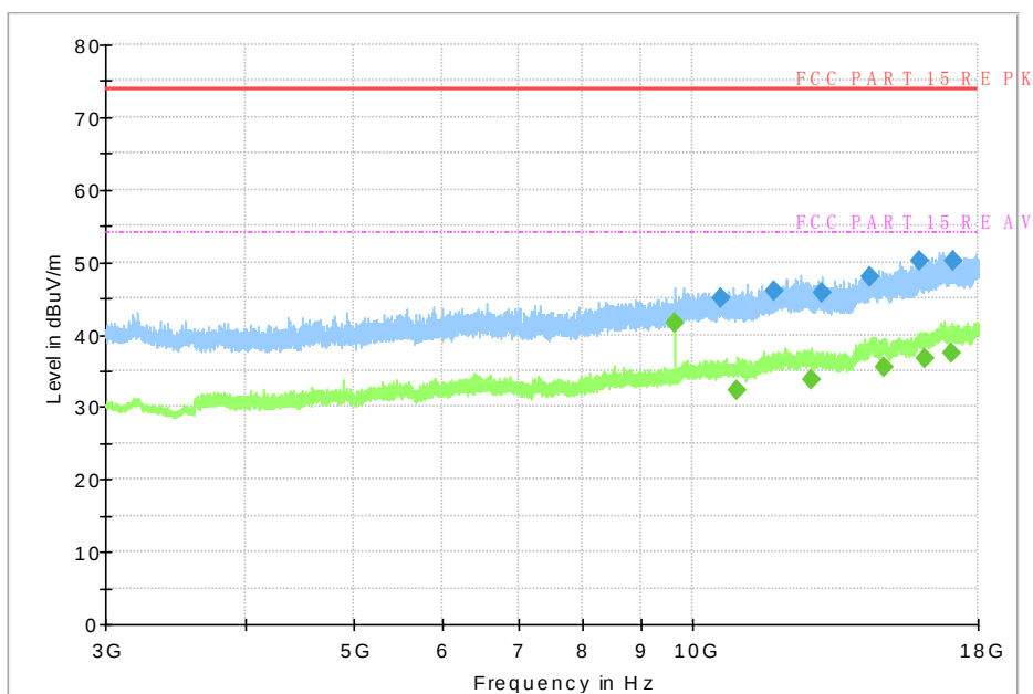
Fig. 56 Radiated Spurious Emission (GFSK, Ch78, 3 GHz ~18 GHz)
