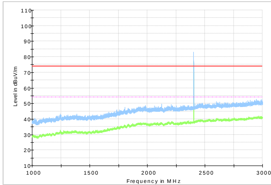
Fig. 67 Radiated Spurious Emission (8DPSK, Ch0, 1 GHz ~3 GHz)
