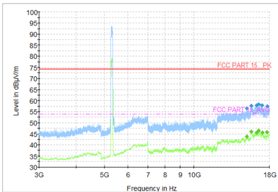
Fig. 108 Transmitter Spurious Emission (802.11ac-VHT80, CH58 5290MHz, 3 GHz-18 GHz)
