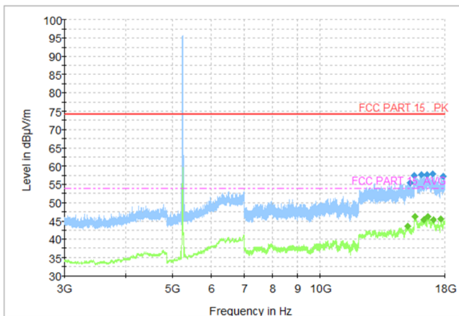
Fig. 68 Transmitter Spurious Emission (802.11a, CH48 5240MHz, 3 GHz-18 GHz)
