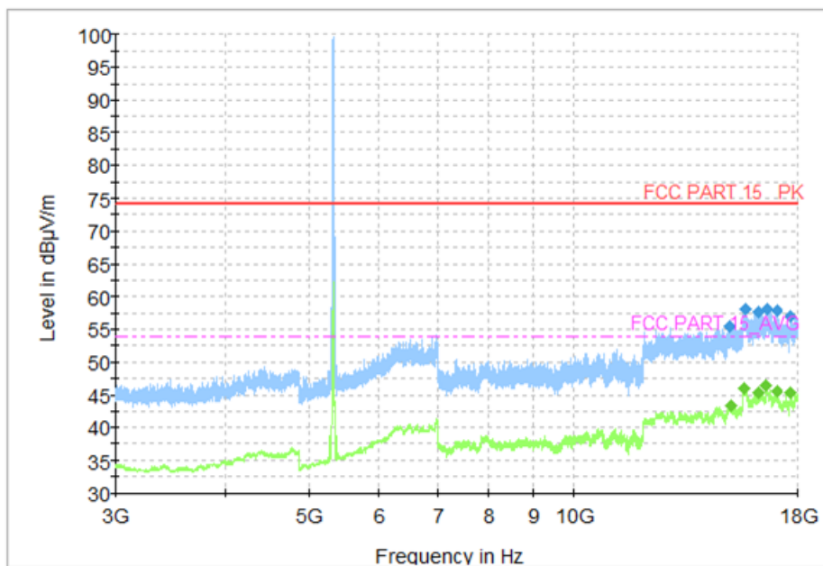
Fig. 74 Transmitter Spurious Emission (802.11a, CH64 5320MHz, 3 GHz-18 GHz)
