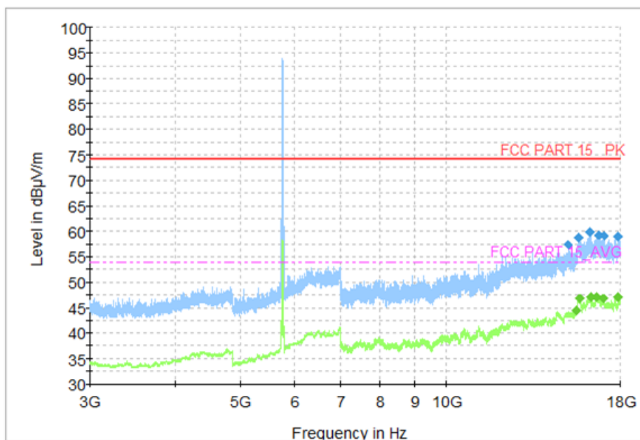
Fig. 102 Transmitter Spurious Emission (802. 11n-HT40, CH151 5755MHz, 3 GHz-18 GHz)
