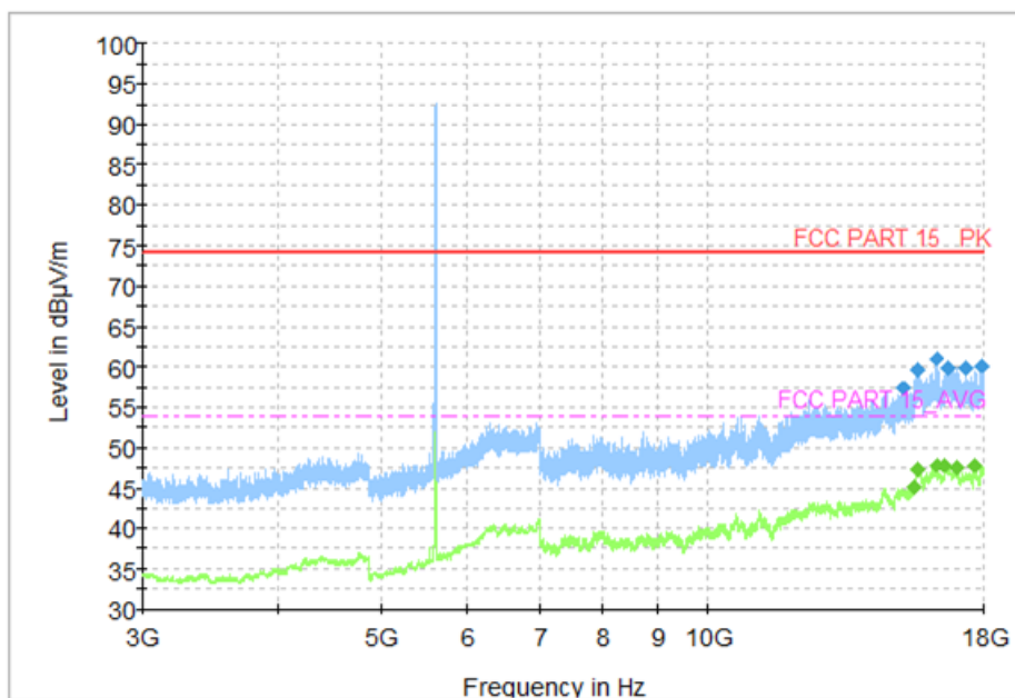
Fig. 78 Transmitter Spurious Emission (802. 11a, CH120 5600MHz, 3 GHz-18 GHz)
