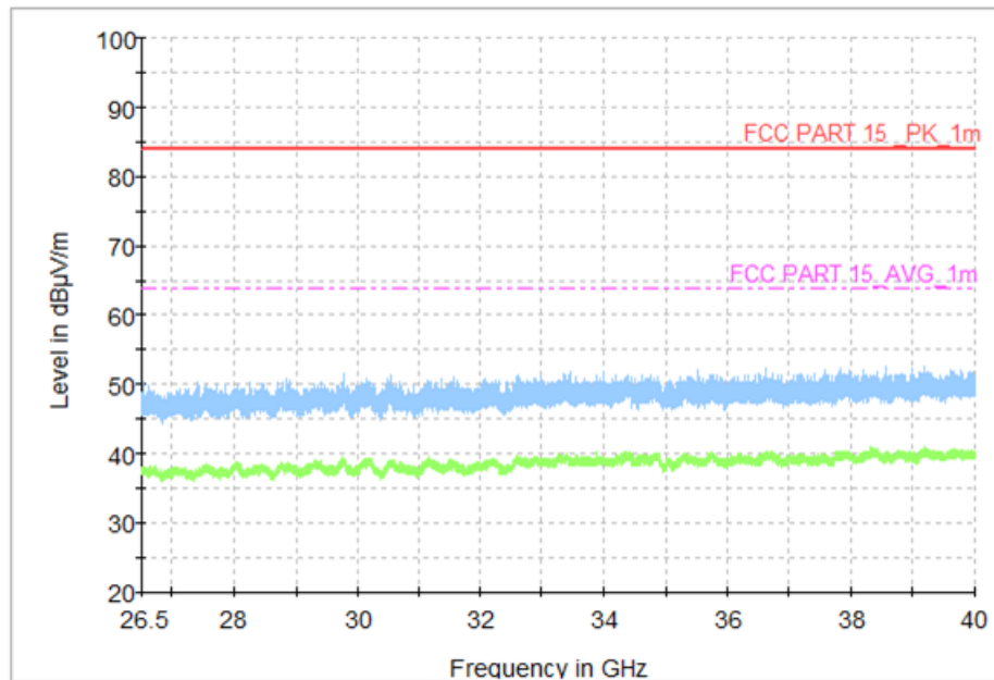
Fig. 117 Transmitter Spurious Emission (All channel, 26.5GHz~40GHz)
