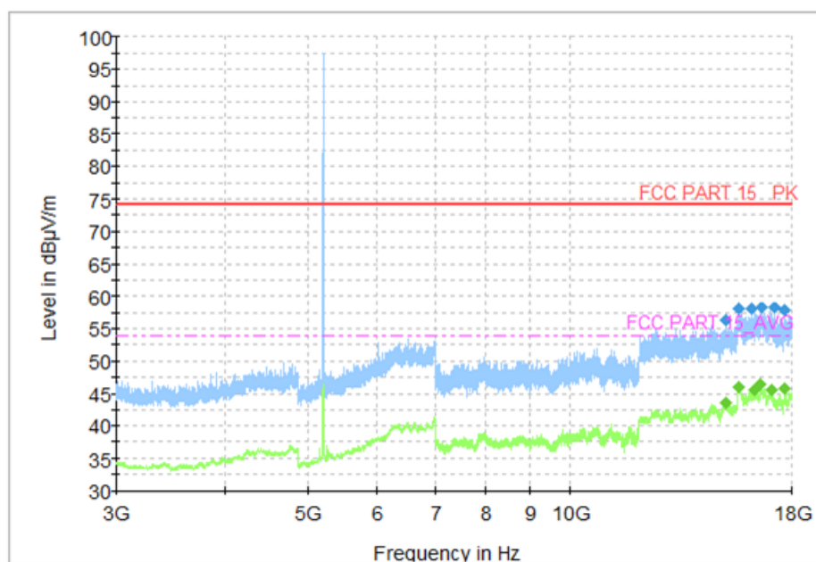
Fig. 66 Transmitter Spurious Emission (802.11a, CH40 5200MHz, 3 GHz-18 GHz)
