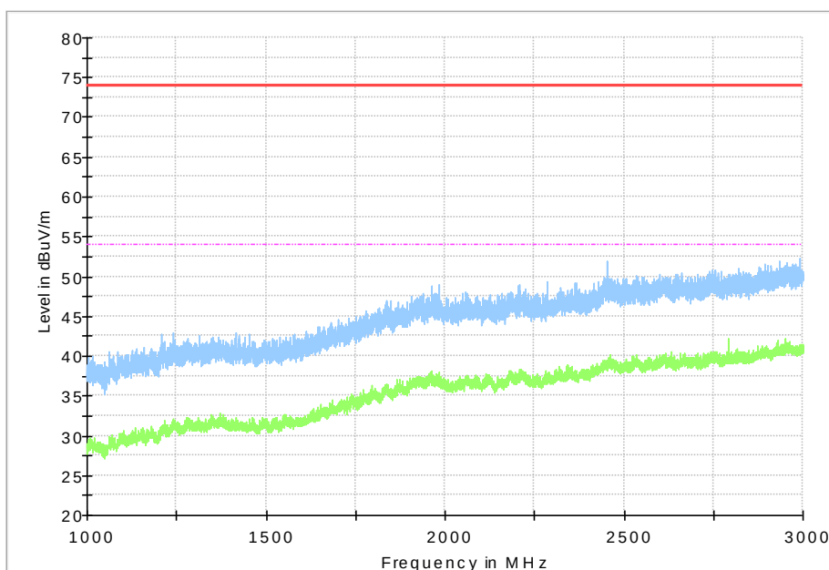
Fig. 109 Transmitter Spurious Emission (802.11ac-VHT80, CH106 5530MHz, 1 GHz-3 GHz)
