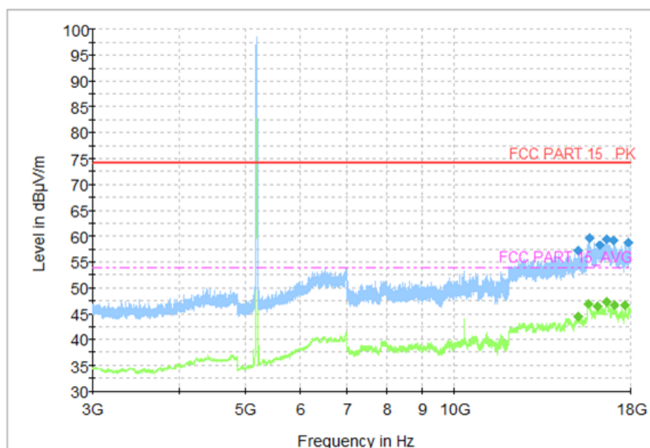
Fig. 64 Transmitter Spurious Emission (802.11a, CH36 5180MHz, 3 GHz-18 GHz)
