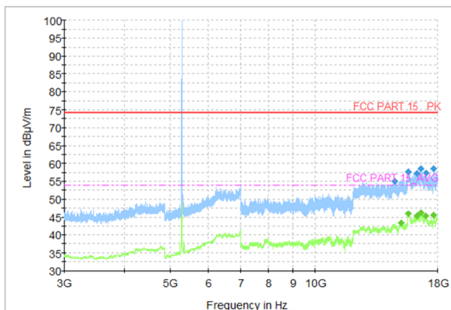
Fig. 72 Transmitter Spurious Emission (802.11a, CH56 5280MHz, 3 GHz-18 GHz)
