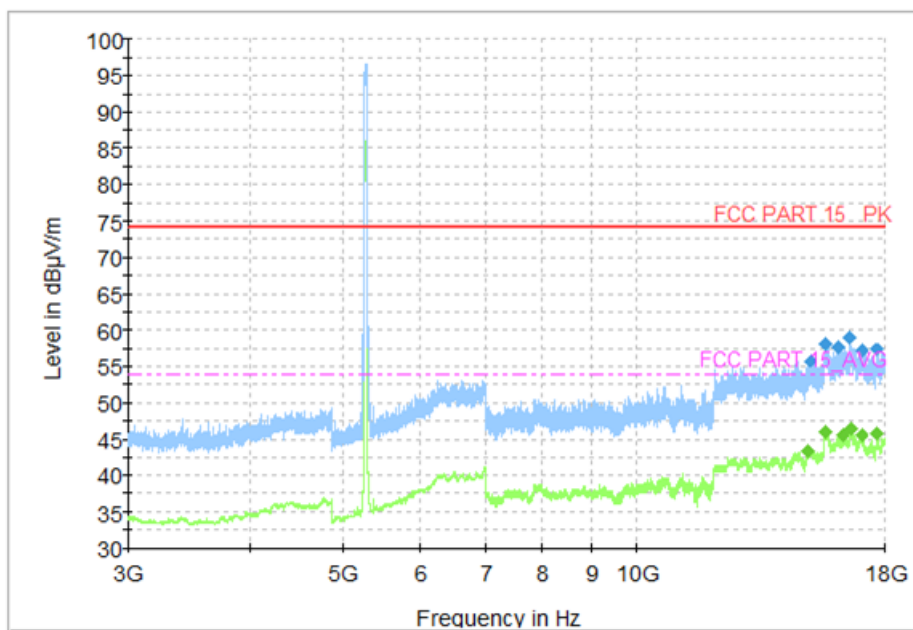
Fig. 94 Transmitter Spurious Emission (802.11n-HT40, CH62 5310MHz, 3 GHz-18 GHz)
