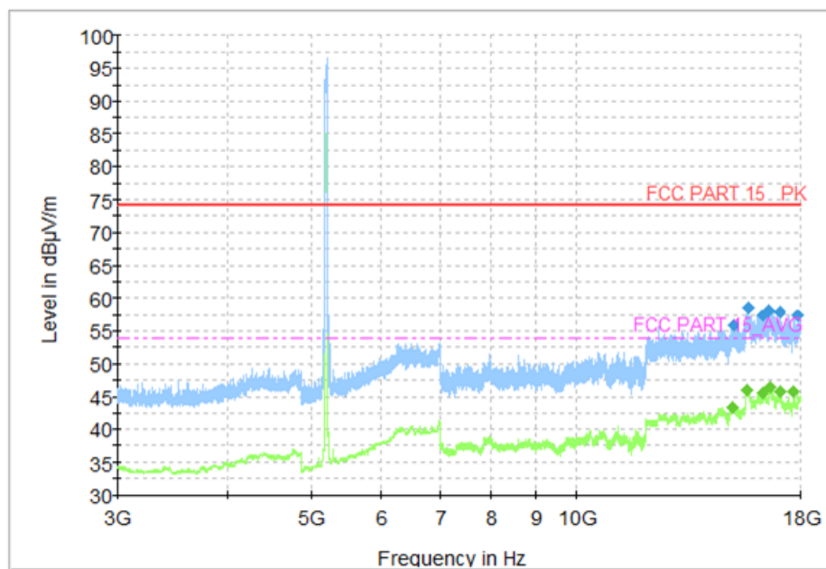
Fig. 88 Transmitter Spurious Emission (802.11n-HT40, CH38 5190MHz, 3 GHz-18 GHz)
