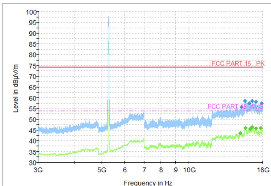
Fig. 92 Transmitter Spurious Emission (802.11n-HT40, CH54 5270MHz, 3 GHz-18 GHz)
