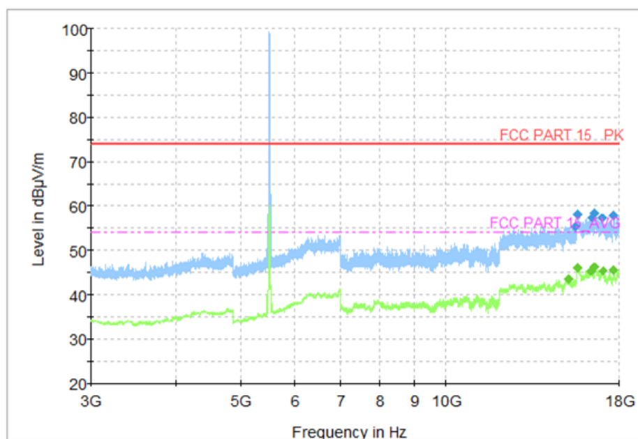
Fig. 76 Transmitter Spurious Emission (802.11a, CH100 5500MHz, 3 GHz-18 GHz)
