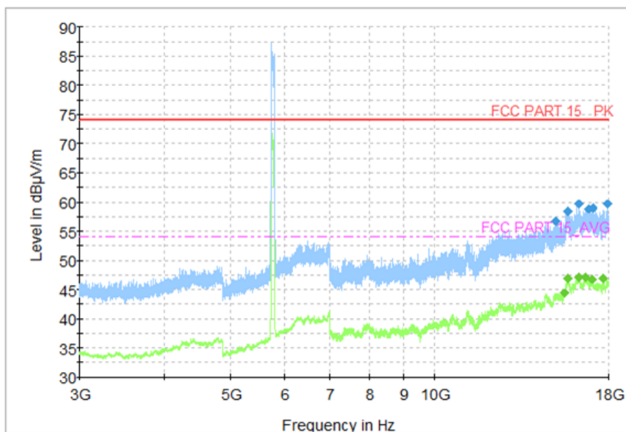
Fig. 114 Transmitter Spurious Emission (802.11ac-VHT80, CH155 5775MHz, 3 GHz-18 GHz)
