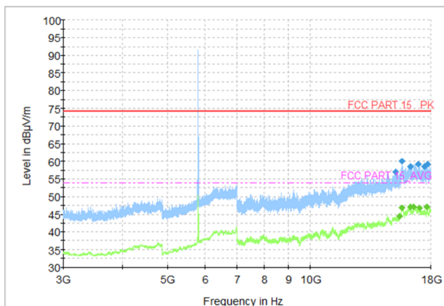
Fig. 104 Transmitter Spurious Emission (802.11n-HT40, CH159 5795MHz, 3 GHz-18 GHz)
