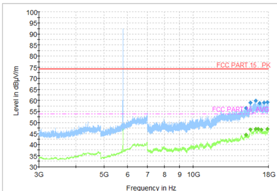
Fig. 84 Transmitter Spurious Emission (802. 11a, CH157 5785MHz, 3 GHz-18 GHz)
