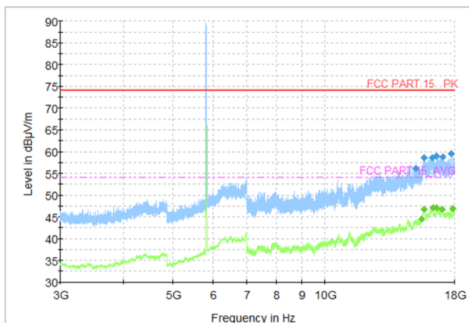
Fig. 86 Transmitter Spurious Emission (802.11a, CH165 5825MHz, 3 GHz-18 GHz)
