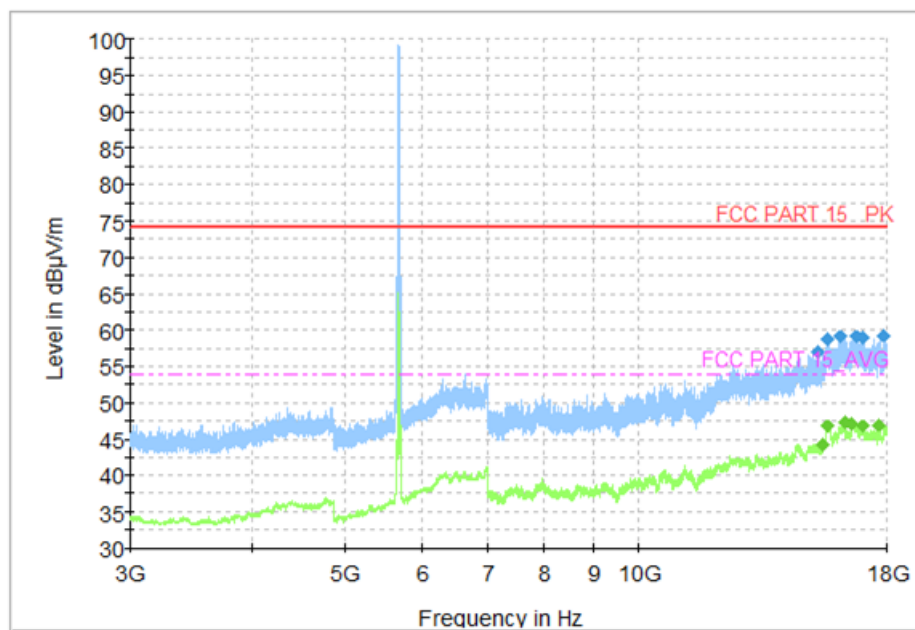
Fig. 100 Transmitter Spurious Emission (802.11n-HT40, CH134 5670MHz, 3 GHz-18 GHz)
