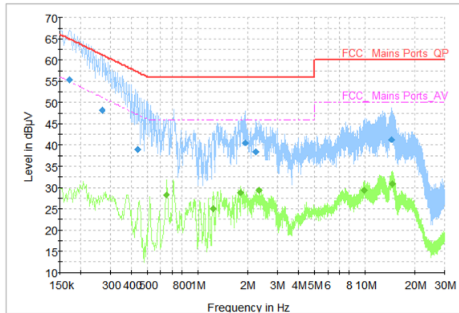
Fig.81 AC Power line Conducted Emission (Idle)
