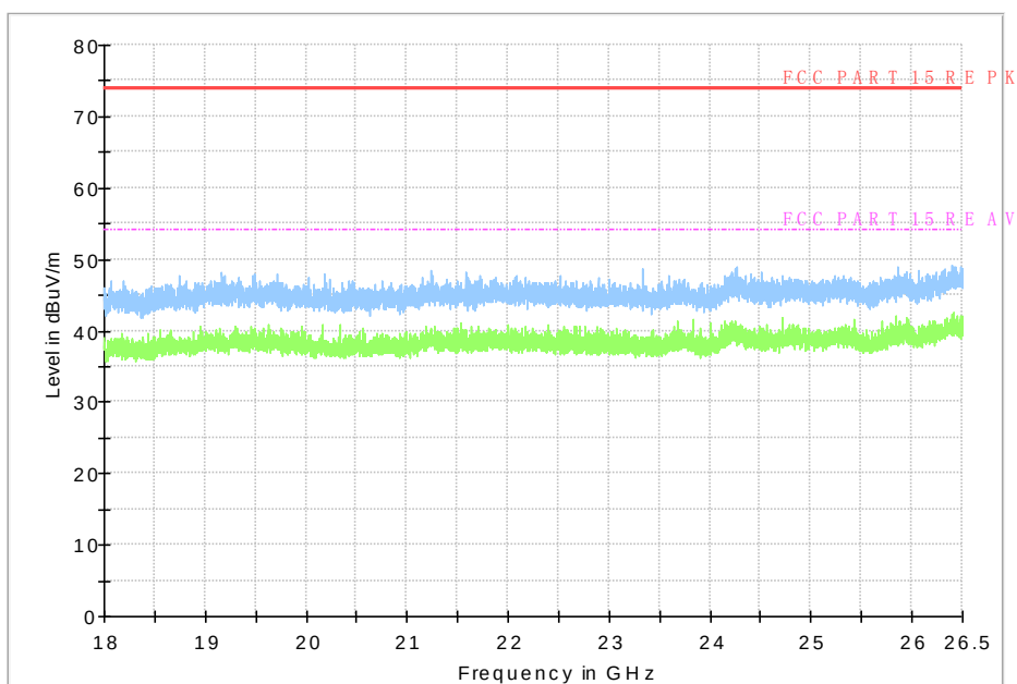
Fig.79 Radiated Spurious Emission (All Channels, 18 GHz-26.5 GHz)
