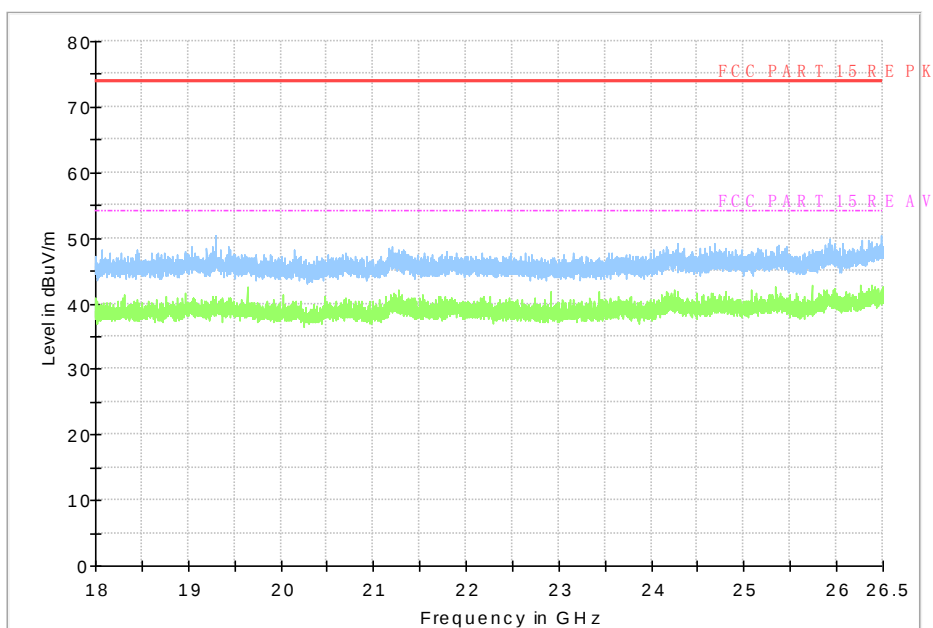
Fig.30 Radiated Spurious Emission (All Channels, 18 GHz-26.5 GHz)
