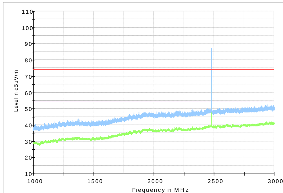
Fig.24 Radiated Spurious Emission (GFSK, Ch39, 1 GHz ~3 GHz)
