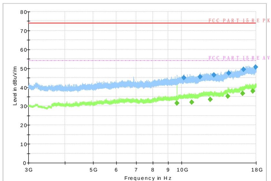
Fig.25 Radiated Spurious Emission (GFSK, Ch39, 3 GHz ~18 GHz)
