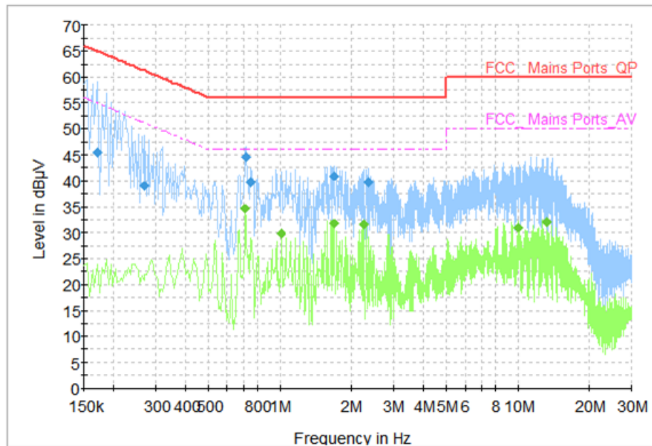
Fig.32 AC Power line Conducted Emission (Idle)
