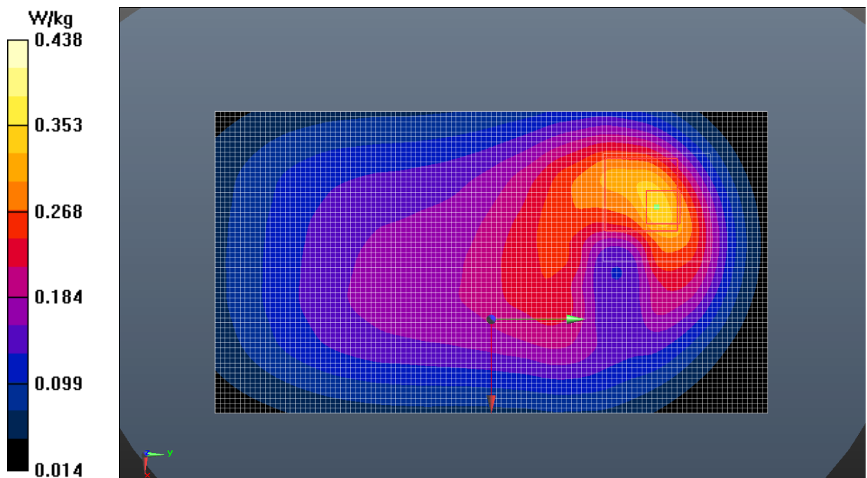
Fig.28 LTE Band 13
