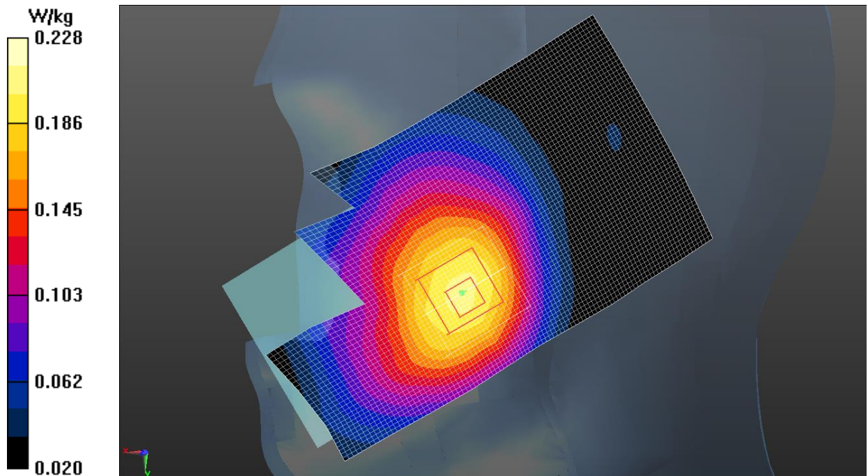
Fig.31 LTE Band 26
