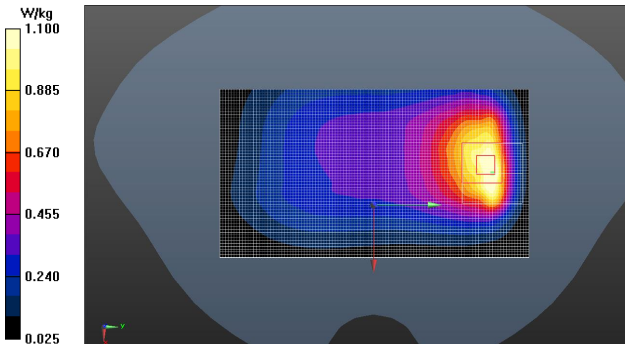
Fig.36 LTE Band 66
