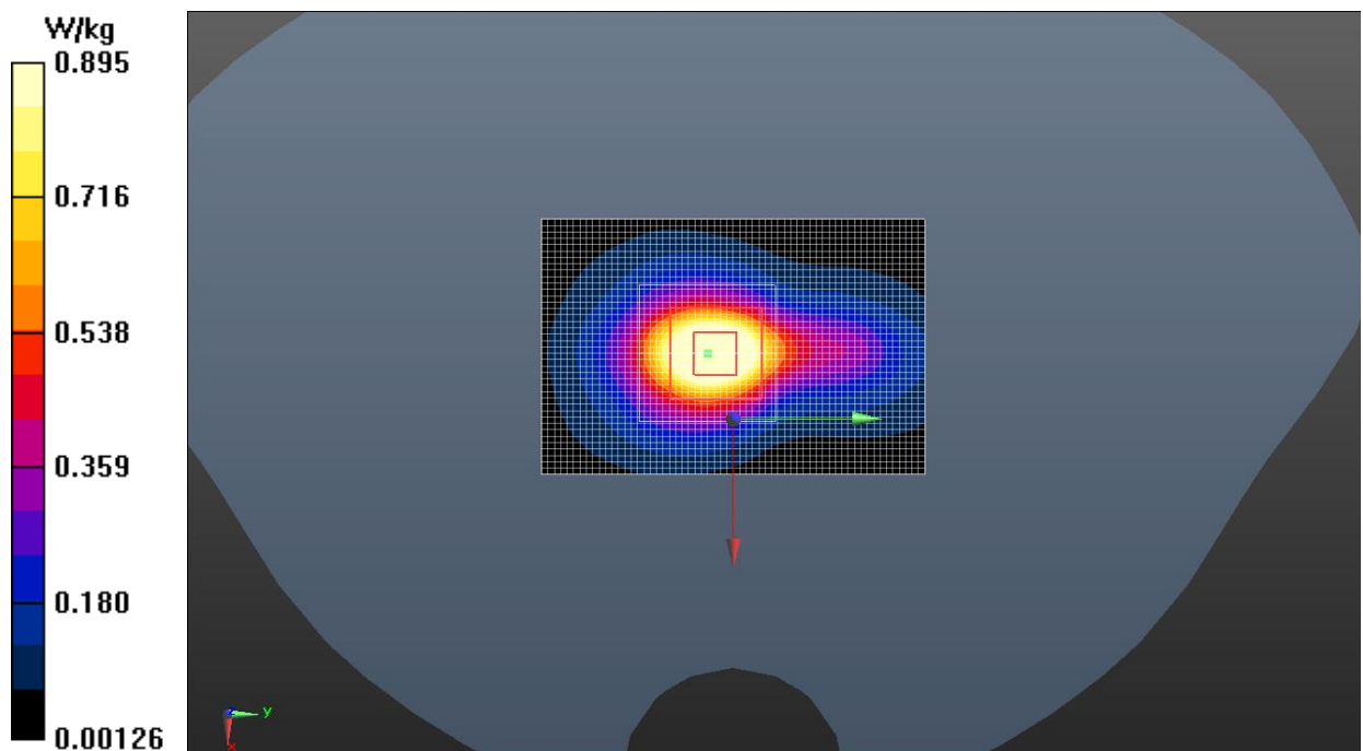
Fig.34 LTE Band 41
