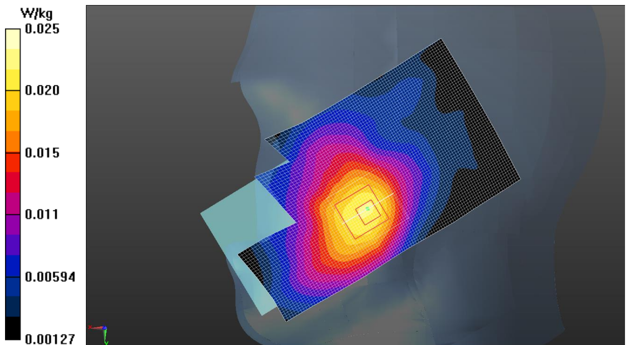
Fig.37 LTE Band 71
