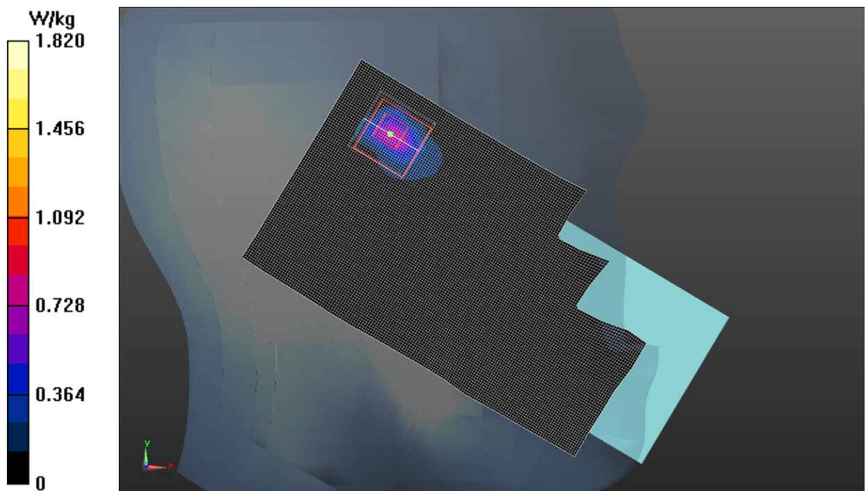
Fig.41 Wi-Fi 5G
