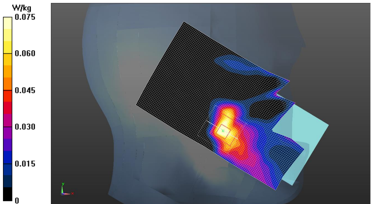
Fig.33 LTE Band 41
