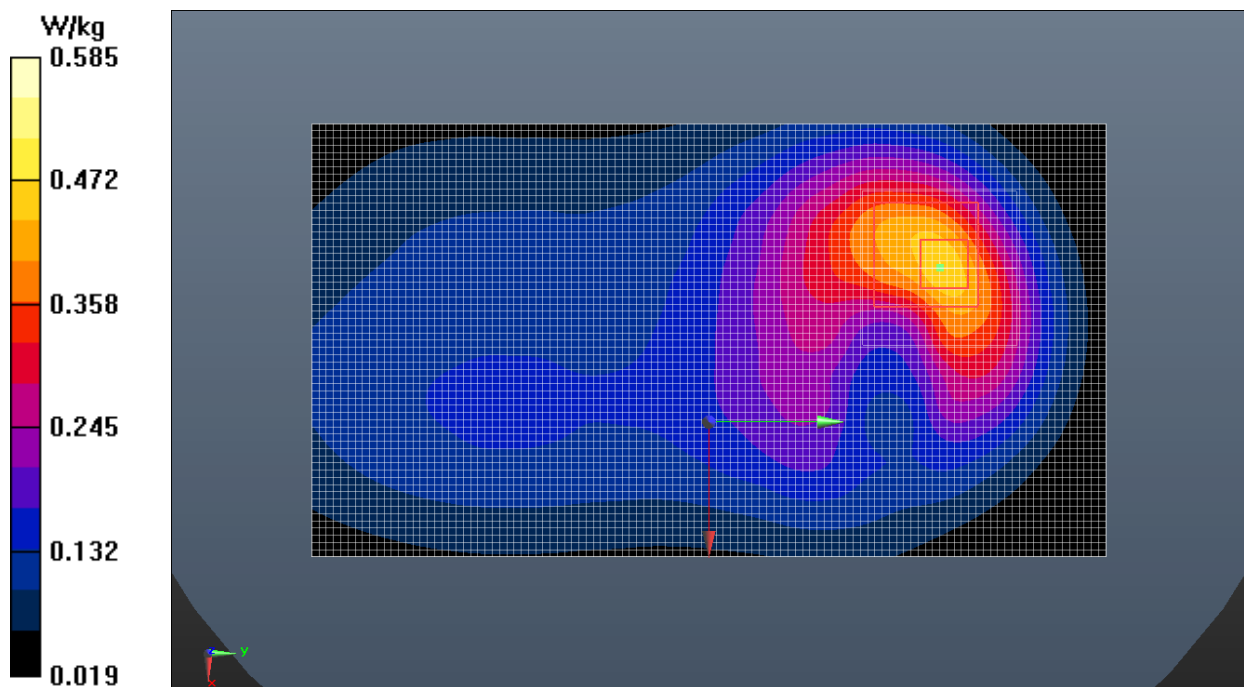
Fig.32 LTE Band 26
