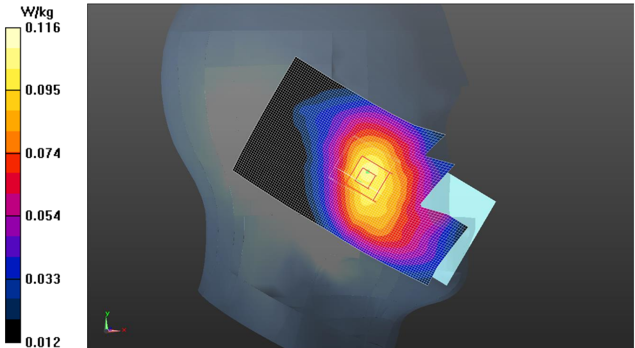
Fig.25 LTE Band 12
