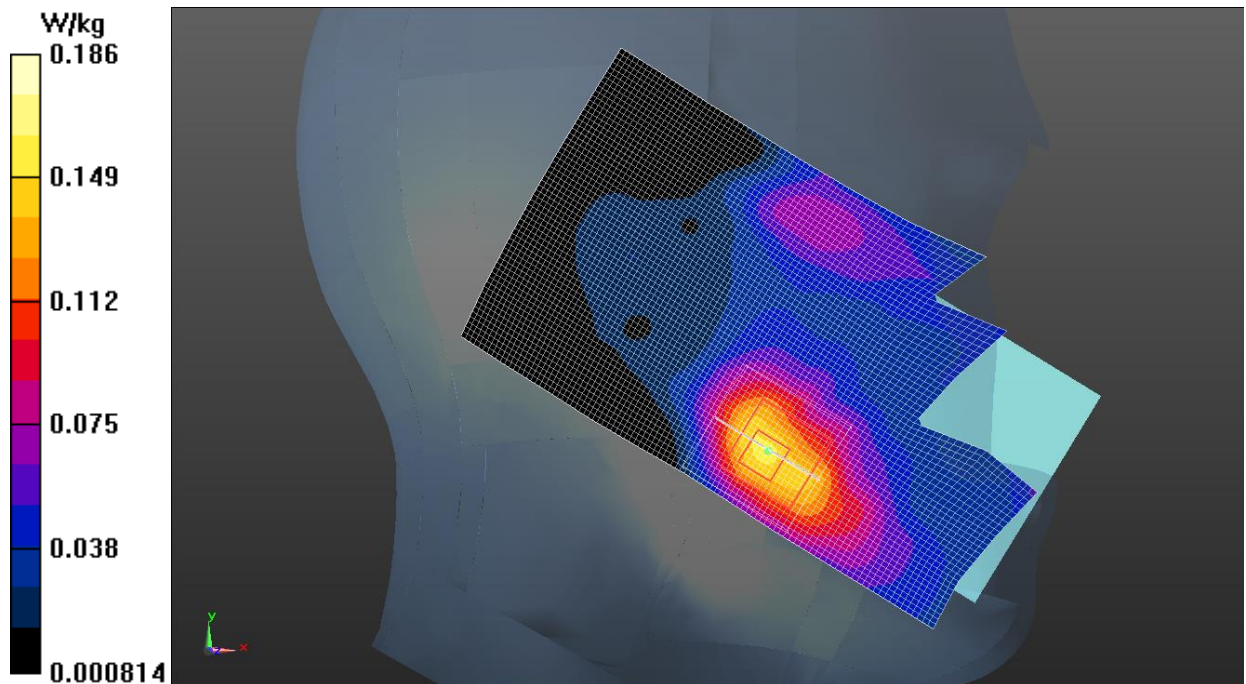
Fig.35 LTE Band 66
