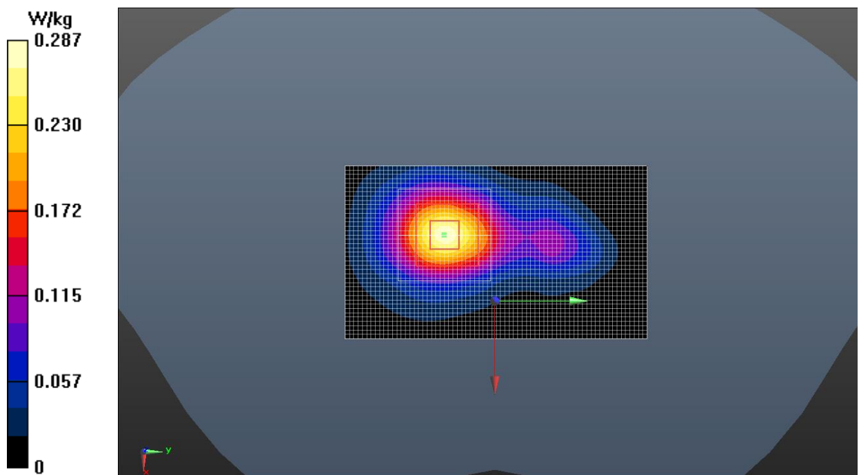
Fig.40 Wi-Fi 2.4G
