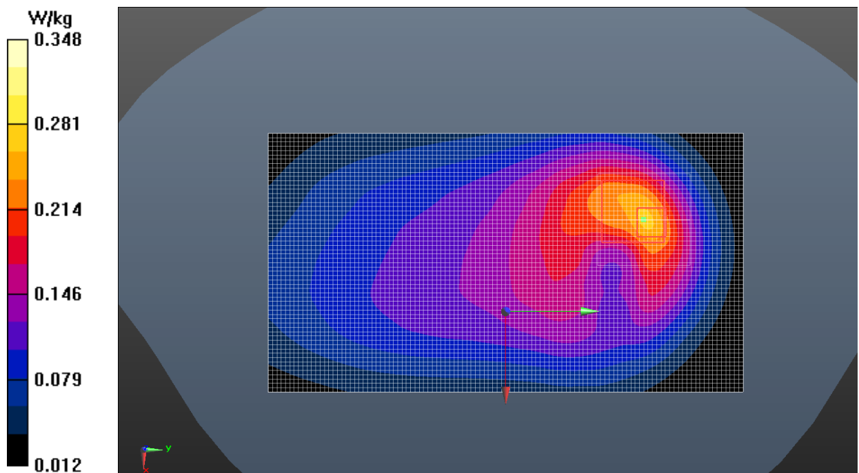
Fig.26 LTE Band 12
