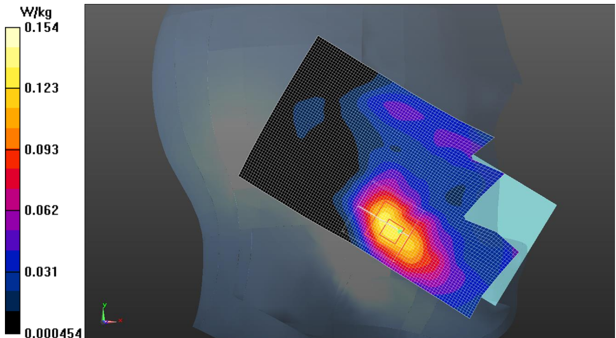
Fig.29 LTE Band 25
