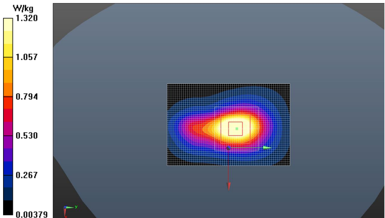
Fig.24 LTE Band 7
