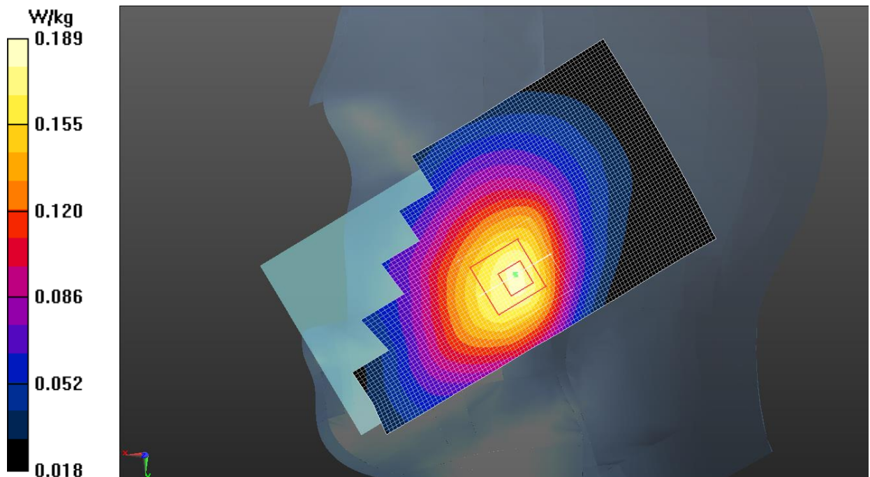
Fig.1 GSM 850
