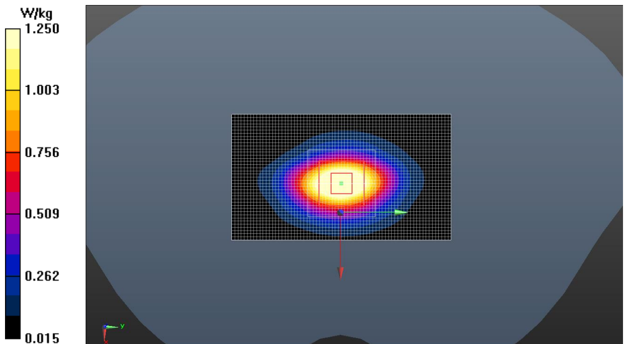
Fig.18 LTE Band 2
