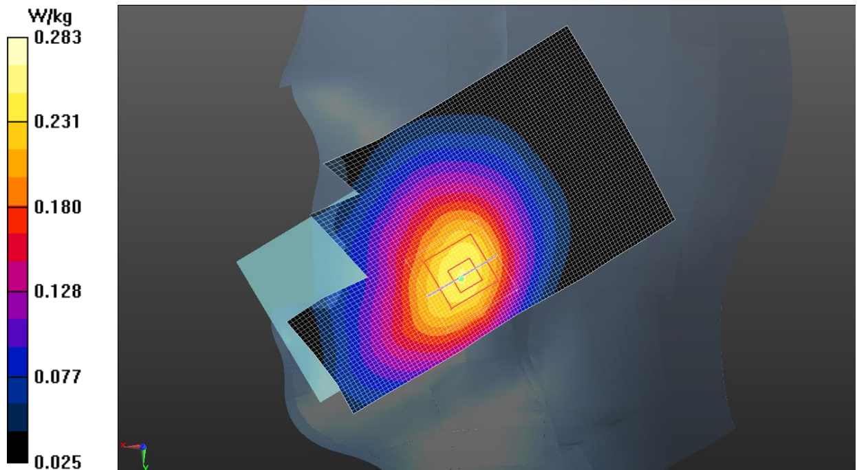
Fig.5 CDMA BC0
