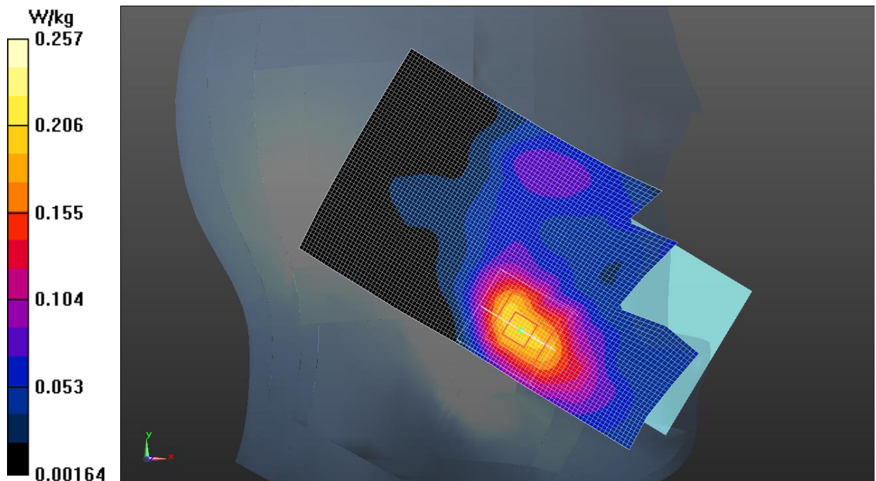
Fig.19 LTE Band 4
