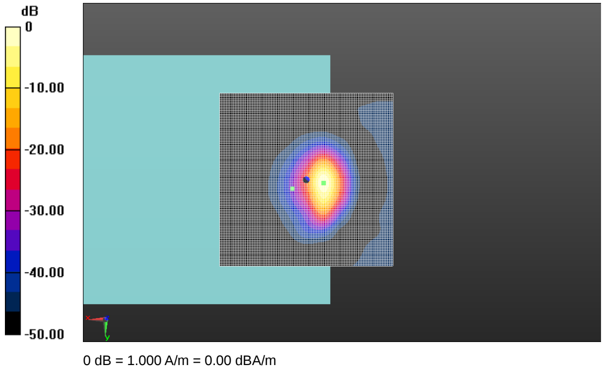
Fig A.26 T-Coil LTE-Band 71-Z
