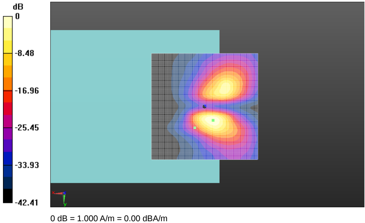
Fig A.26 T-Coil LTE-Band 71-Y
