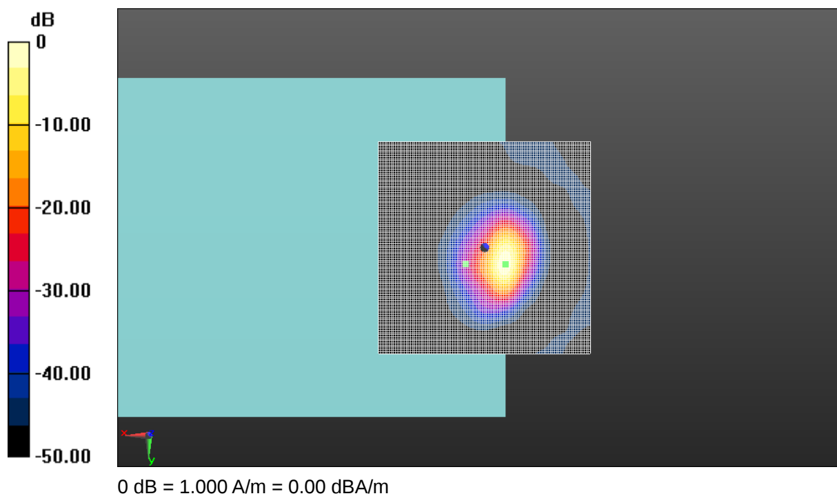
Fig A.12 T-Coil CDMA BC1-Z
