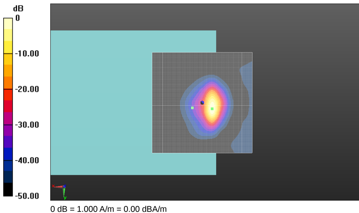
Fig A.18 T-Coil LTE-Band 4-Z
