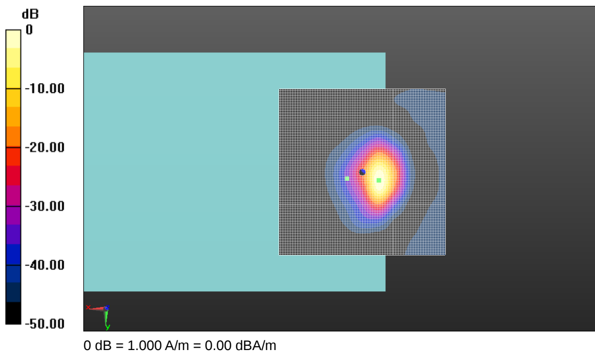
Fig A.20 T-Coil LTE-Band 12-Z
