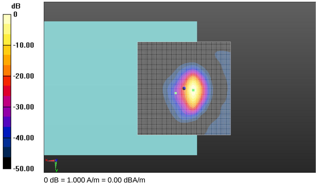
Fig A.25 T-Coil LTE-Band 66-Z
