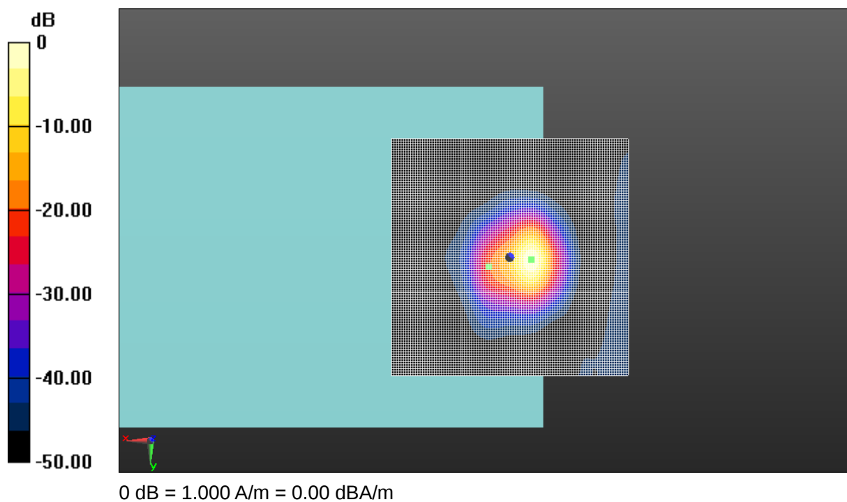
Fig A.24 T-Coil LTE-Band 41-Z
