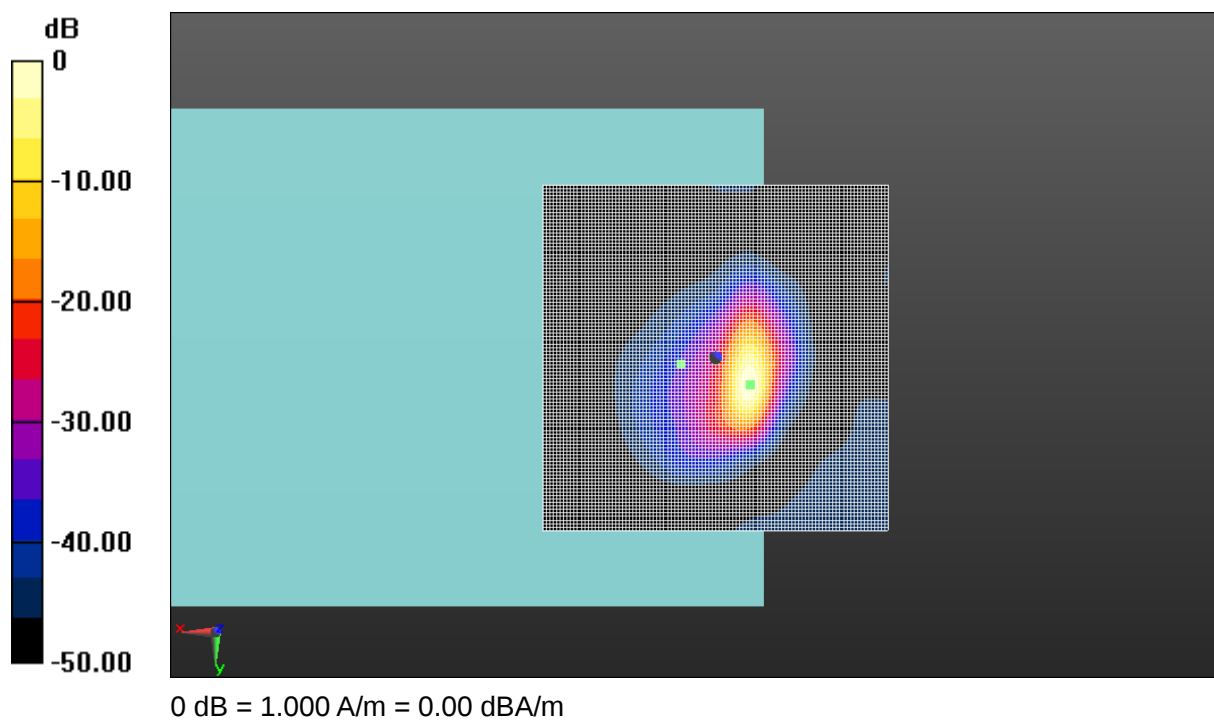
Fig A.27 T-Coil WIFI 2.4G-Z
