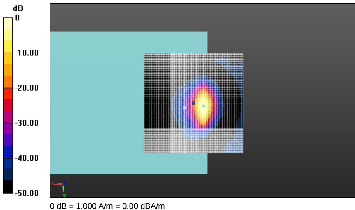
Fig A.21 T-Coil LTE-Band 13-Z
