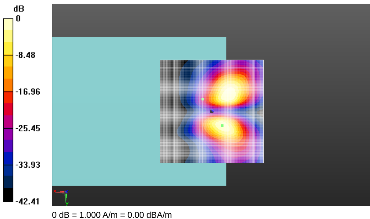
Fig A.23 T-Coil LTE-Band 26-Y
