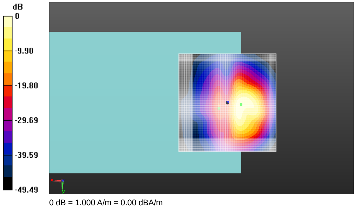
Fig A.10 T-Coil GSM 1900-Z
