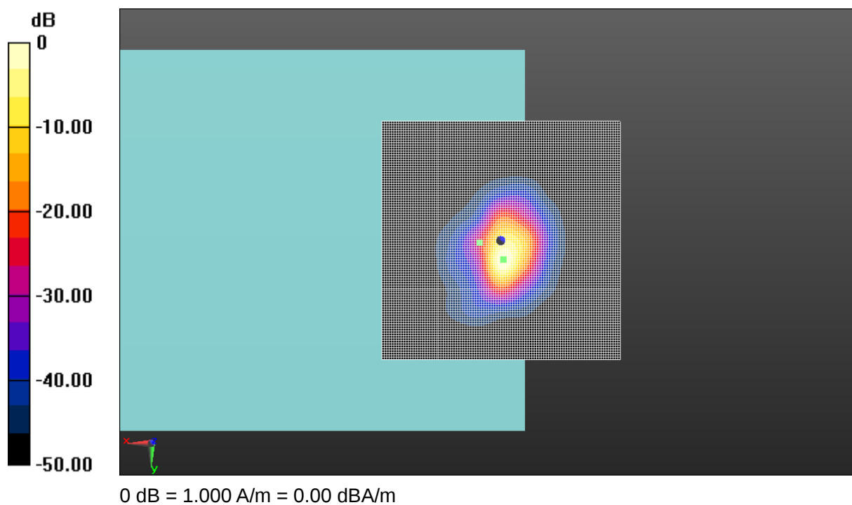
Fig A.4 T-Coil CDMA BC1-Z
