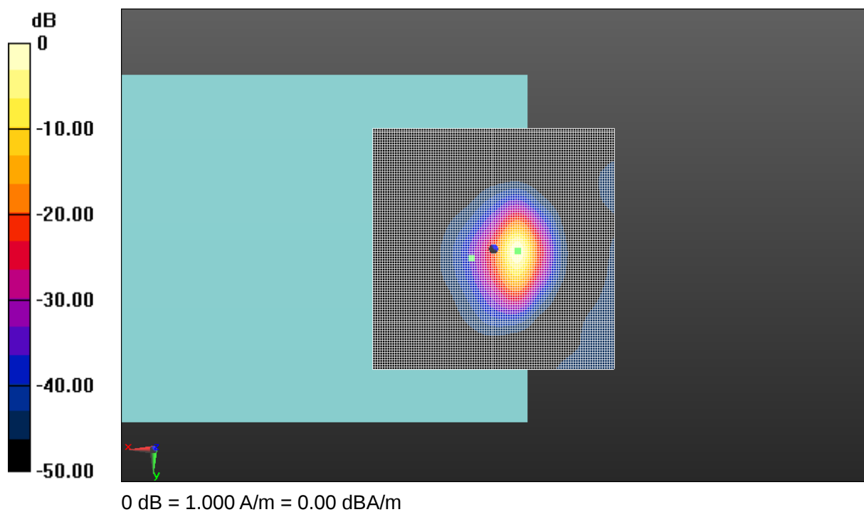
Fig A.22 T-Coil LTE-Band 25-Z
