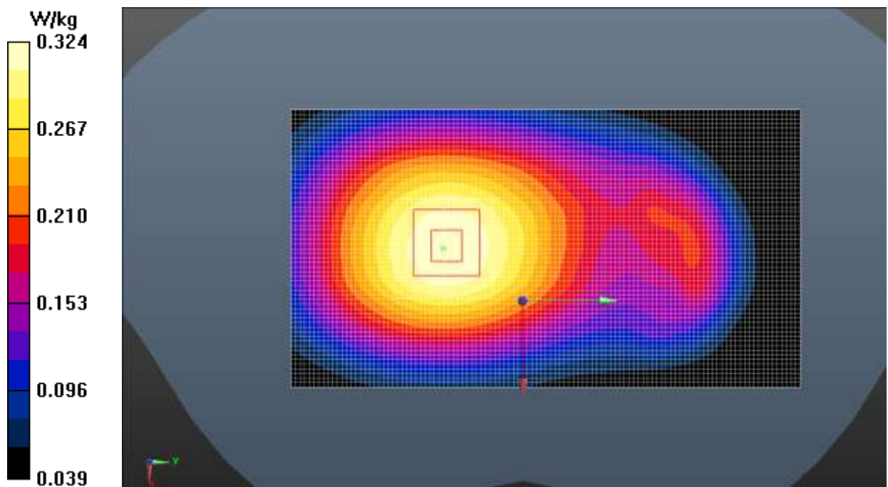
Fig.12 WCDMA 850
