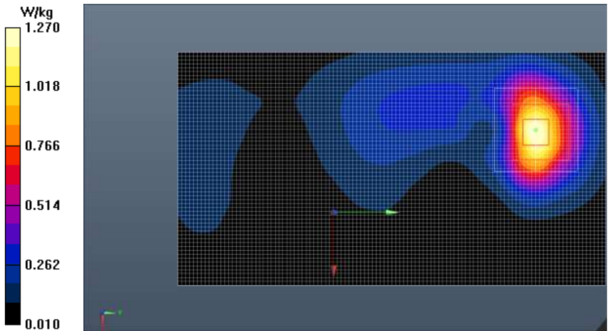
Fig.8 CDMA BC1
