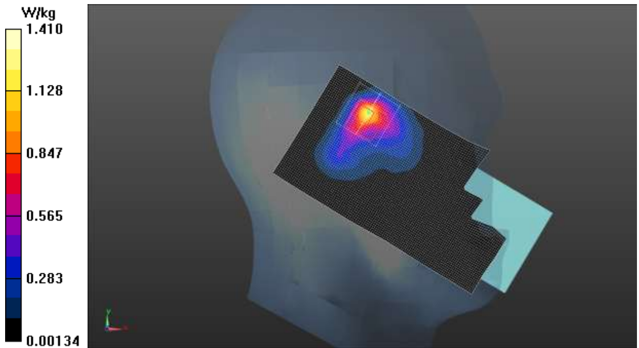
Fig.37 Wi-Fi 2.4G
