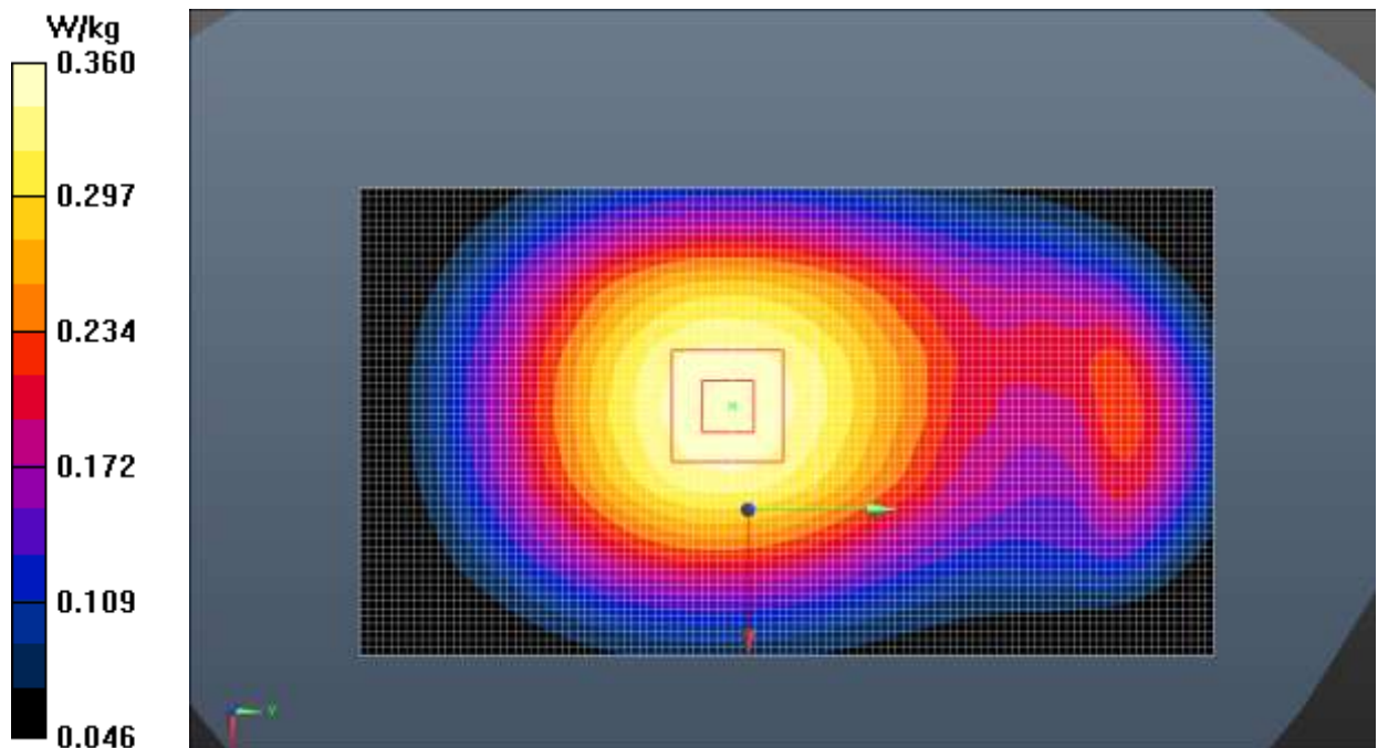
Fig.22 LTE Band 5
