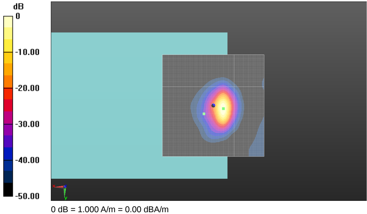
Fig A.33 T-Coil LTE-Band 2
