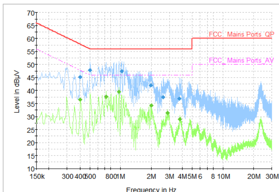
Fig.87 AC Power line Conducted Emission (Idle, AE4, 240V)
