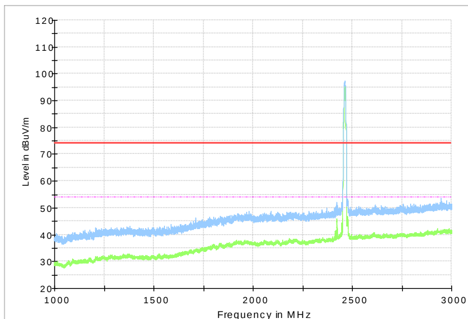
Fig.49 Radiated Spurious Emission (802.11b, CH11, 1GHz-3GHz)
