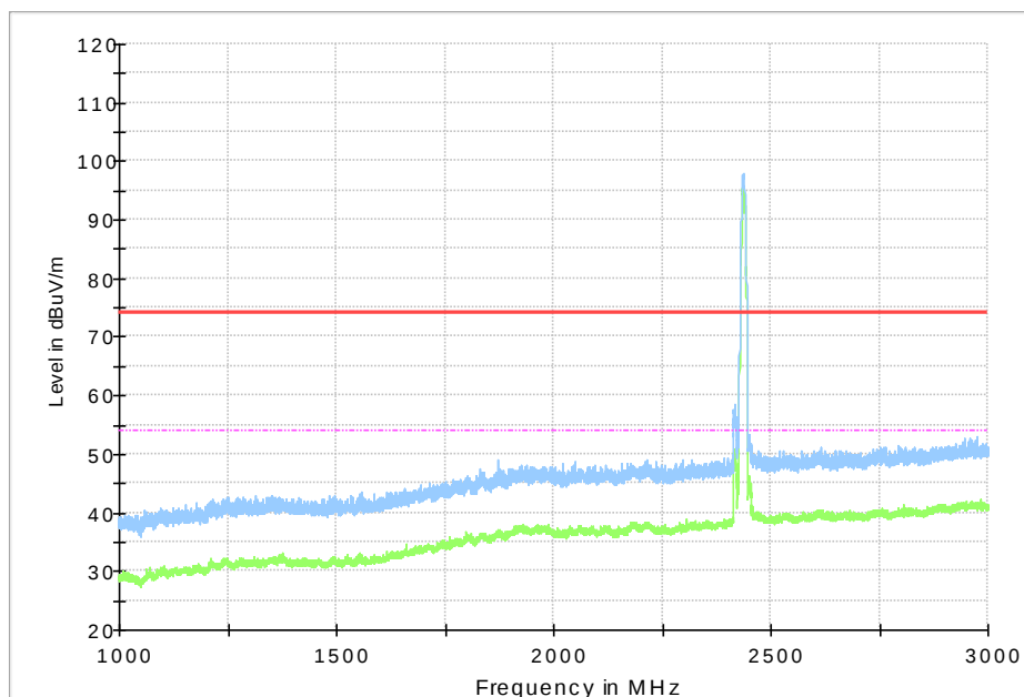
Fig.47 Radiated Spurious Emission (802.11b, CH6, 1GHz-3GHz)
