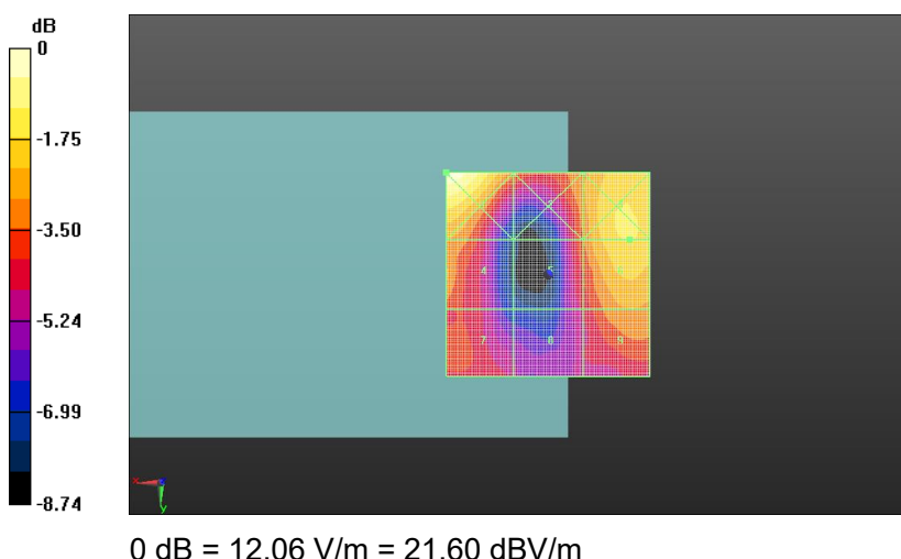
Fig A.8 HAC RF E-Field LTE-Band 41 Middle
