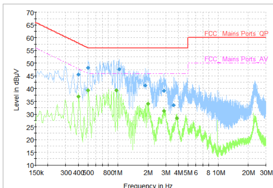
Fig.38 AC Power line Conducted Emission (Idle, AE4, 240V), 1M
