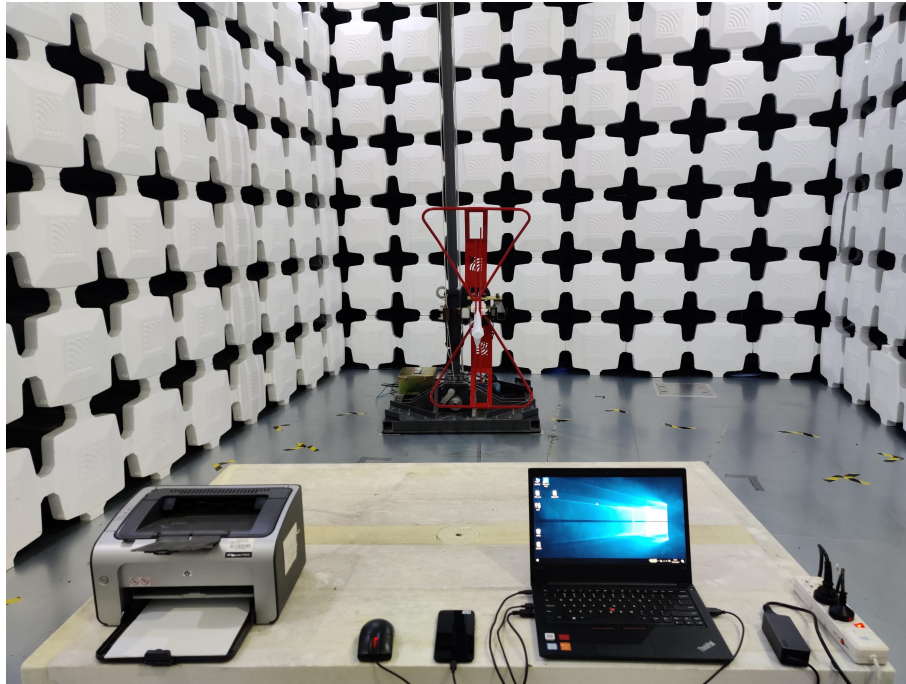
1. Radiated Emissions (Part 15B,Data transfer mode) (30MHz- 1GHz)
