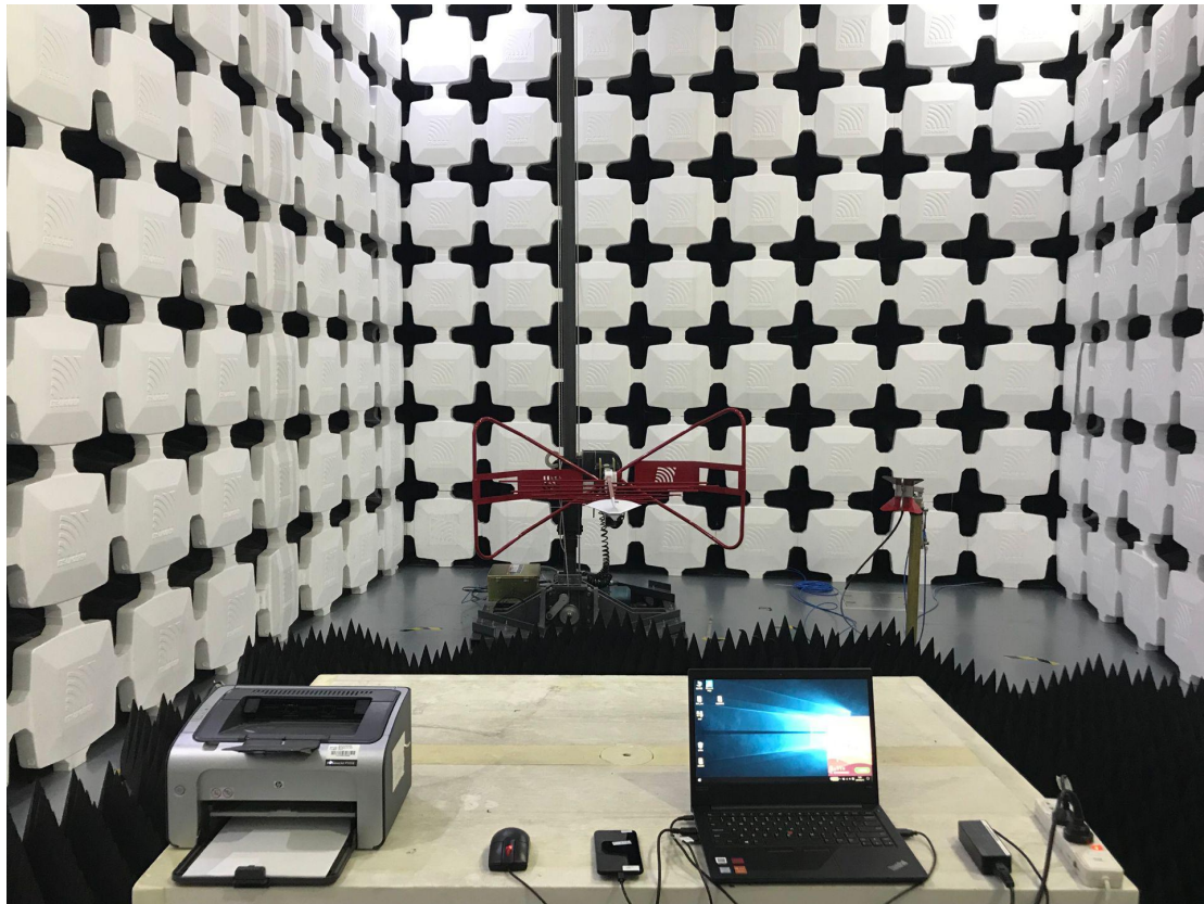
2. Radiated Emissions (Part 15B,Data transfer mode)( 1GHz-18GHz)
